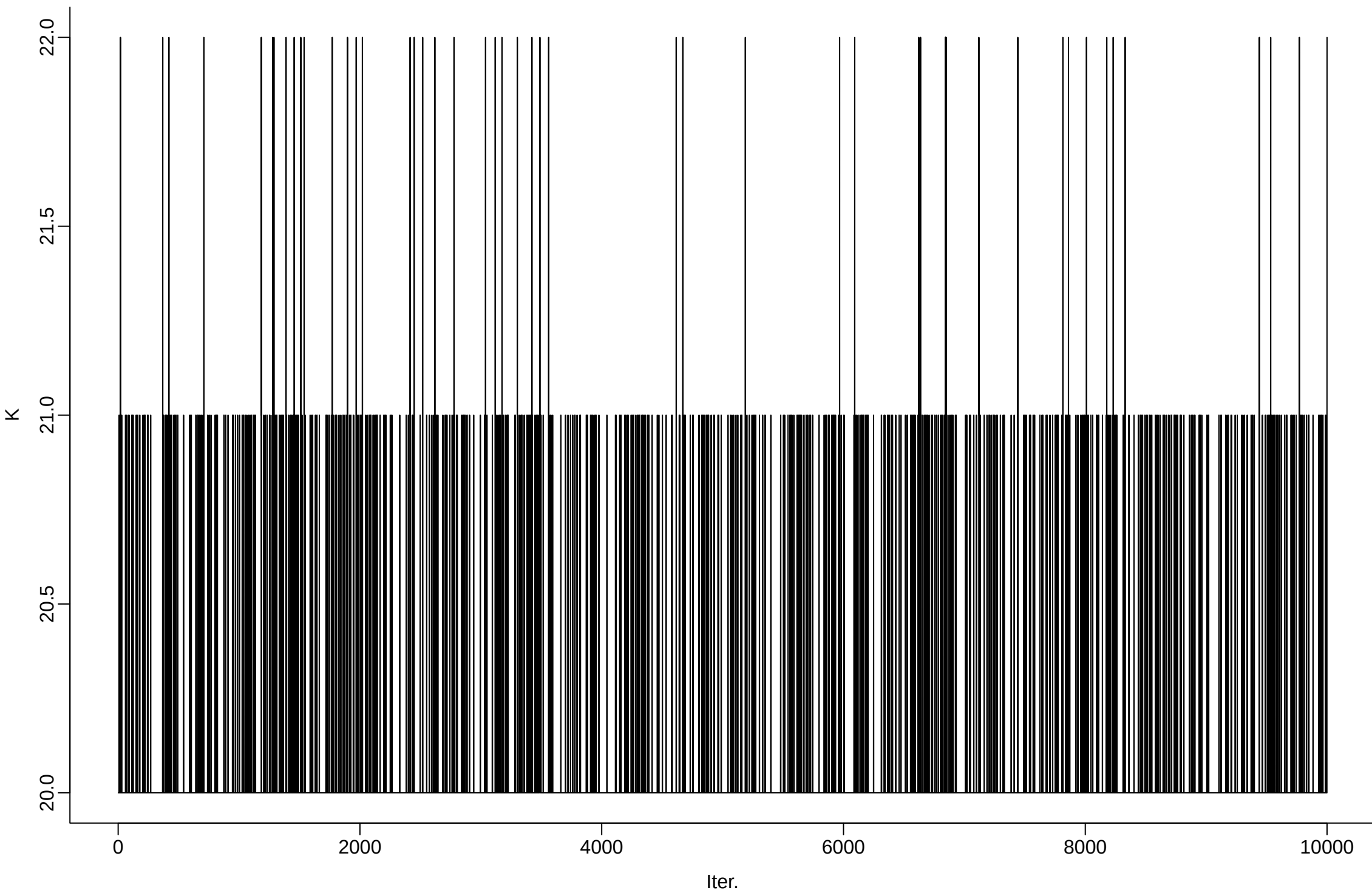
cfg105_r10_delta_1em02_beta0_1e00_gamma0_1em03_sigma0_2p5em01 | Total number of distinct topics
