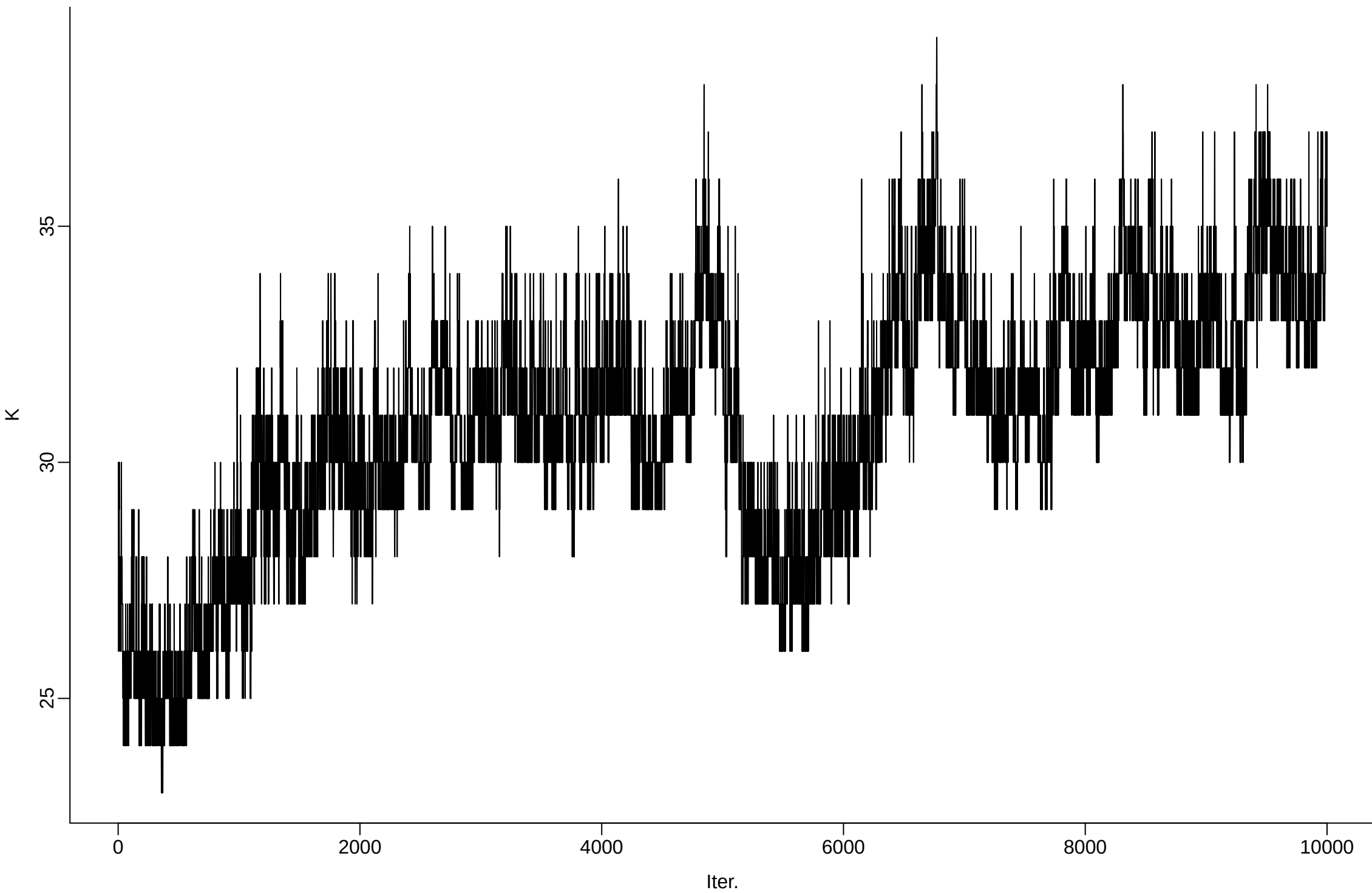
cfg122_r10_delta_1em03_beta0_1em04_gamma0_1em01_sigma0_2p5em01 | Total number of distinct topics
