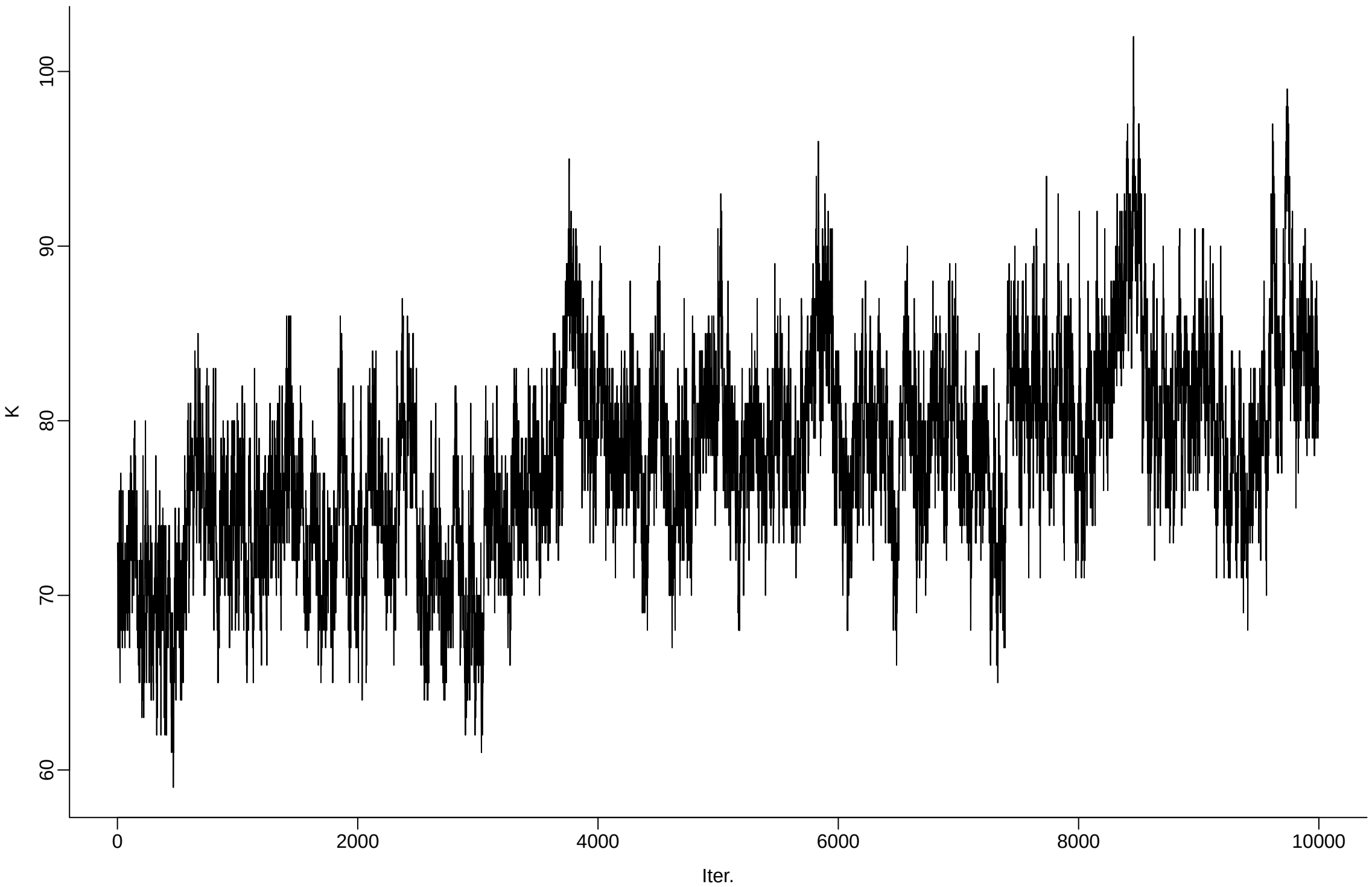
cfg149_r10_delta_1em03_beta0_1e00_gamma0_1e00_sigma0_2p5em01 | Total number of distinct topics
