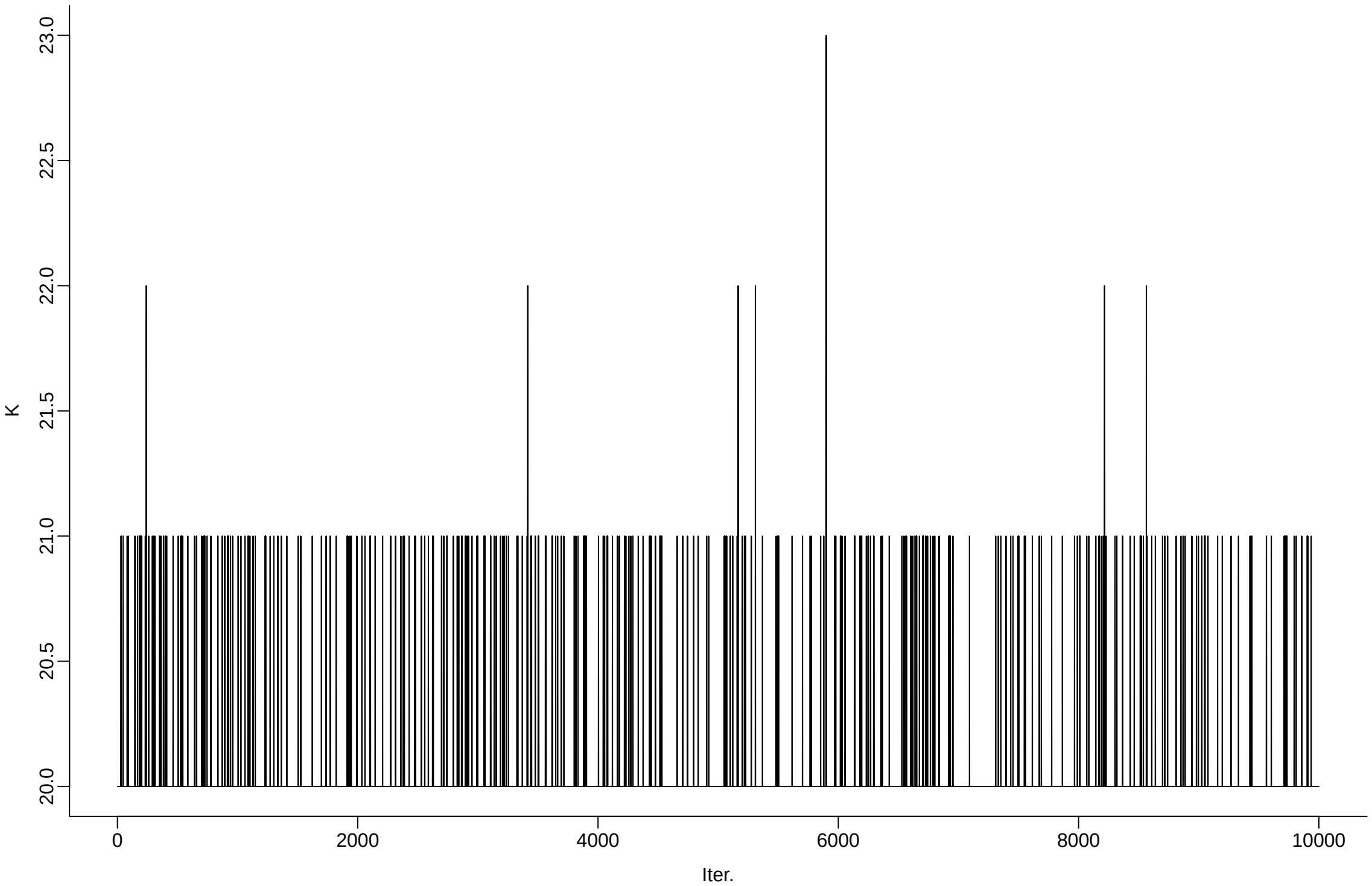
cfg168_r10_delta_1em02_beta0_1em04_gamma0_1em03_sigma0_5em01 | Total number of distinct topics
