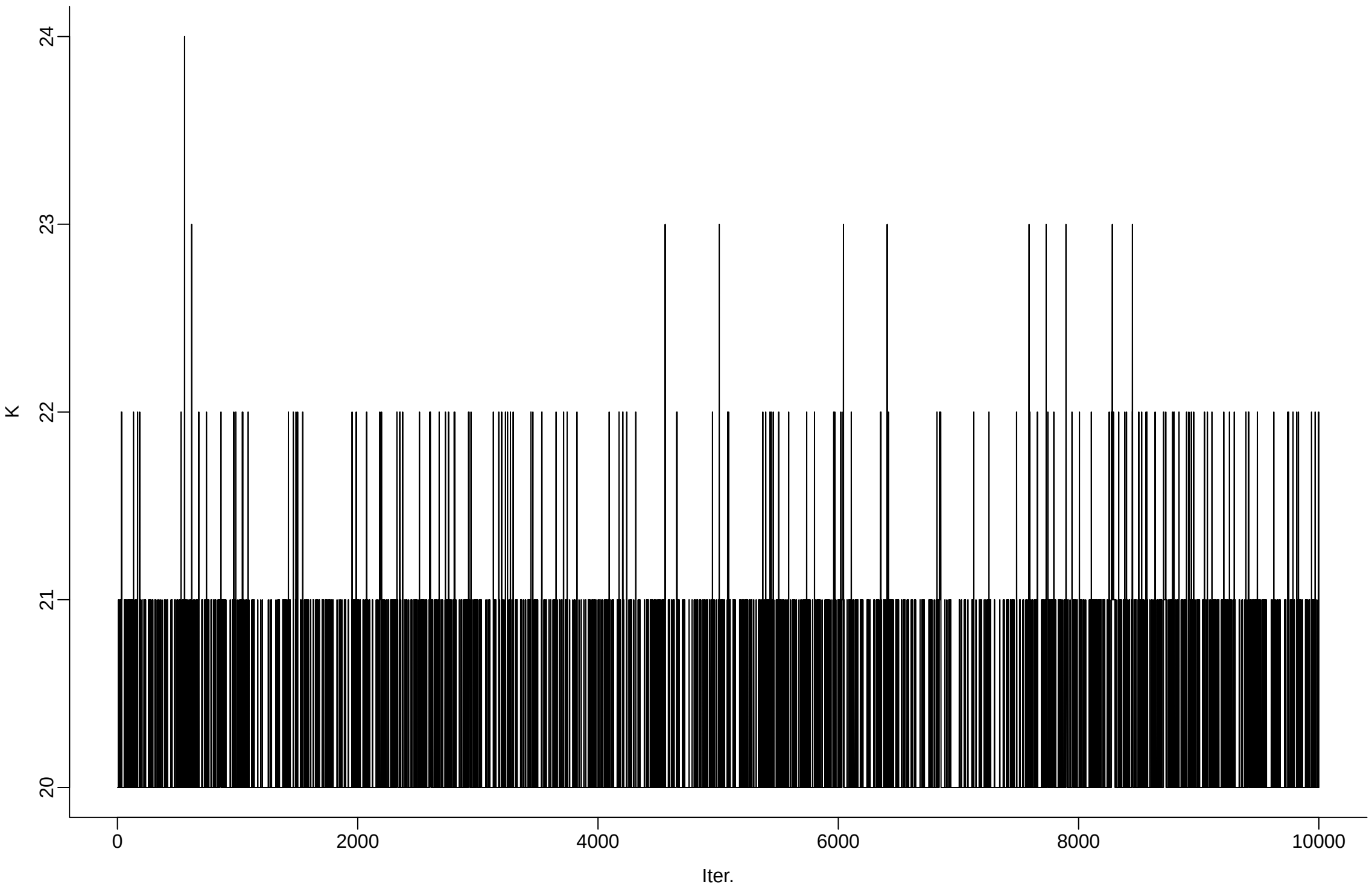
cfg179_r10_delta_1em03_beta0_1e00_gamma0_1em03_sigma0_5em01 | Total number of distinct topics
