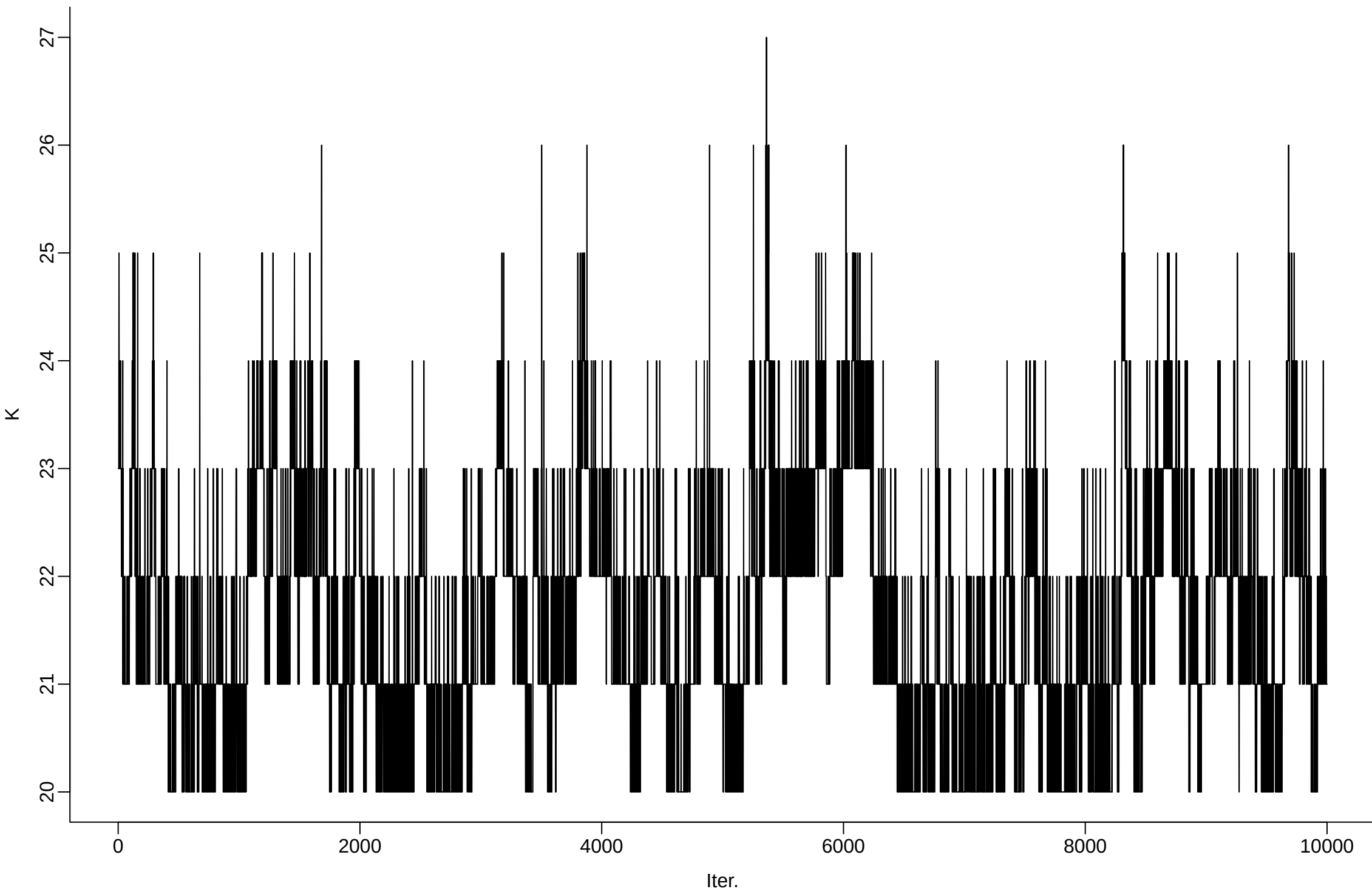
cfg189_r10_delta_1em02_beta0_1em02_gamma0_1em02_sigma0_5em01 | Total number of distinct topics
