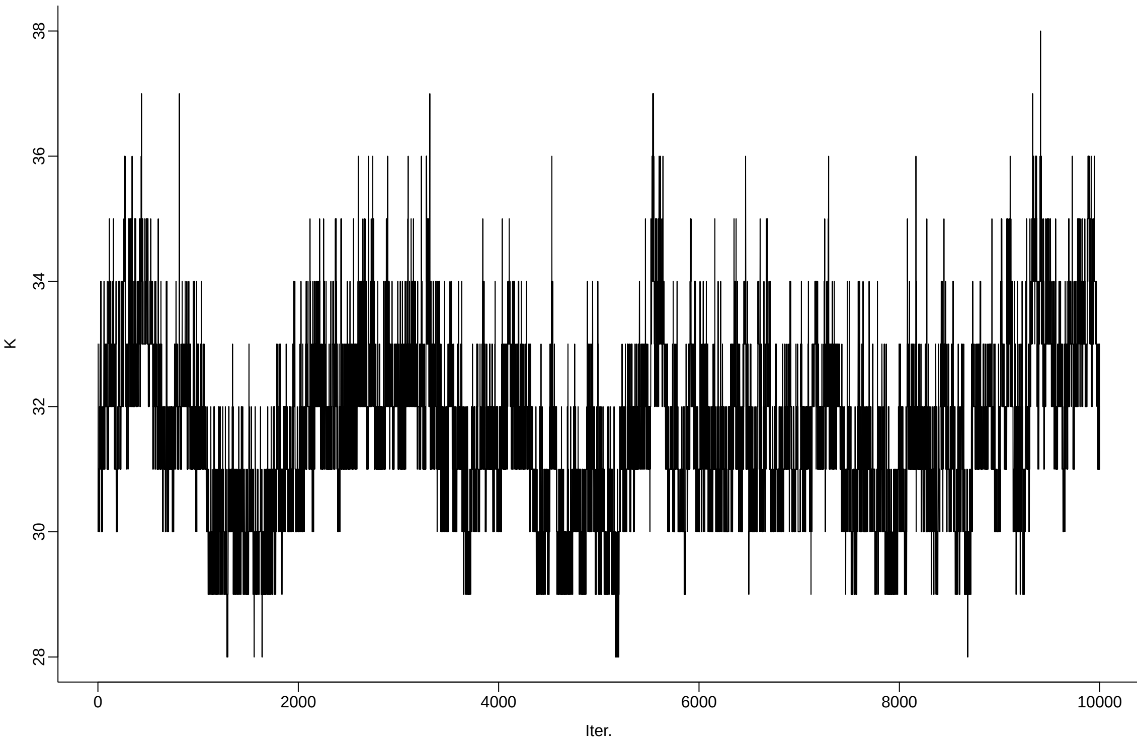
cfg203_r10_delta_1em03_beta0_1em02_gamma0_1em01_sigma0_5em01 | Total number of distinct topics
