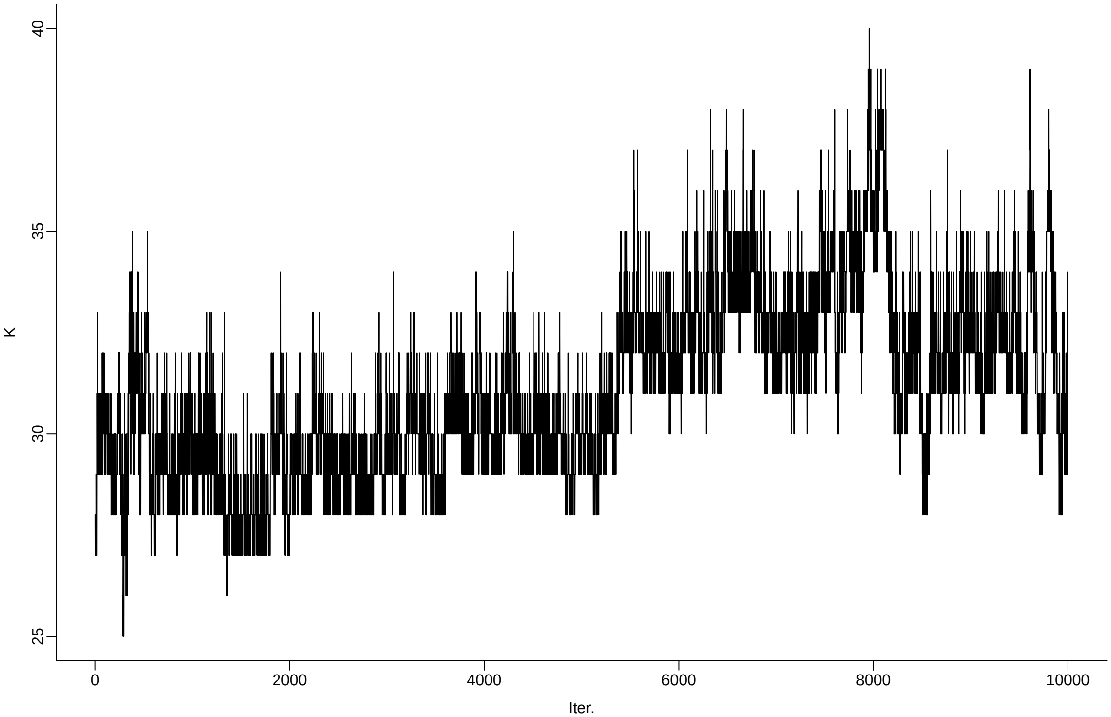
cfg206_r10_delta_1em03_beta0_1em01_gamma0_1em01_sigma0_5em01 | Total number of distinct topics
