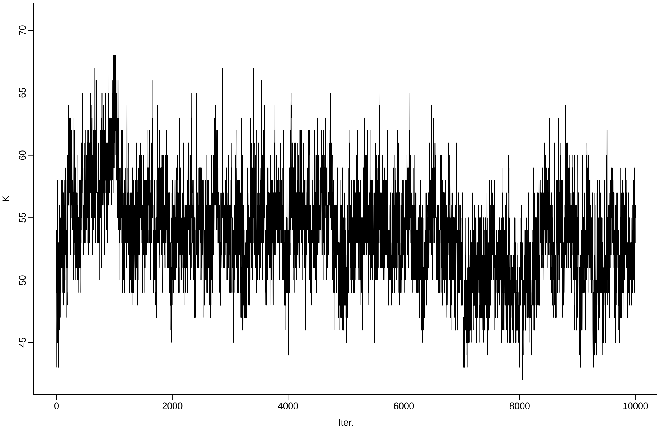
cfg215_r10_delta_1em03_beta0_1em03_gamma0_1e00_sigma0_5em01 | Total number of distinct topics
