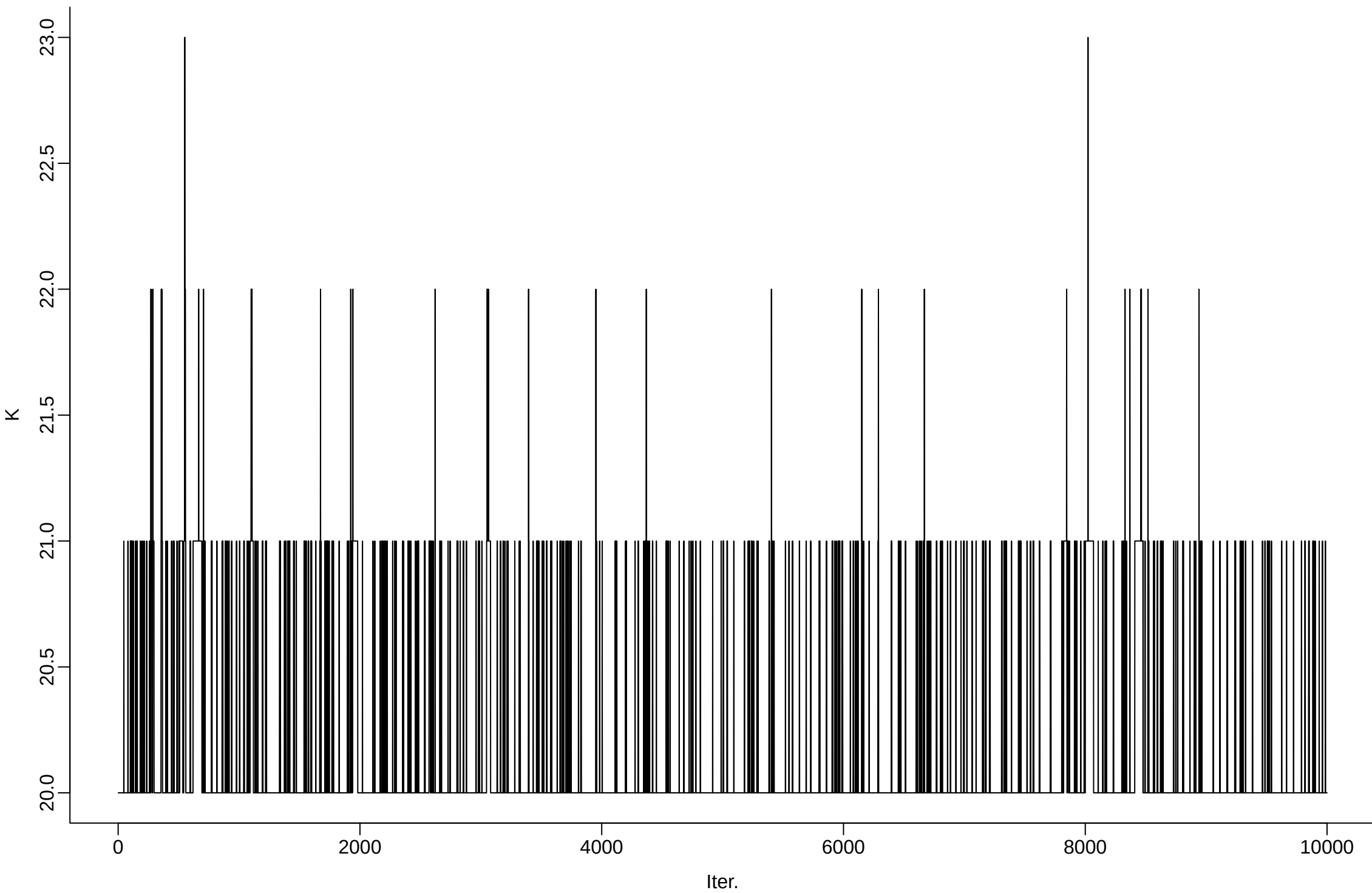
cfg248_r10_delta_1em03_beta0_1em02_gamma0_1em03_sigma0_7p5em01 | Total number of distinct topics
