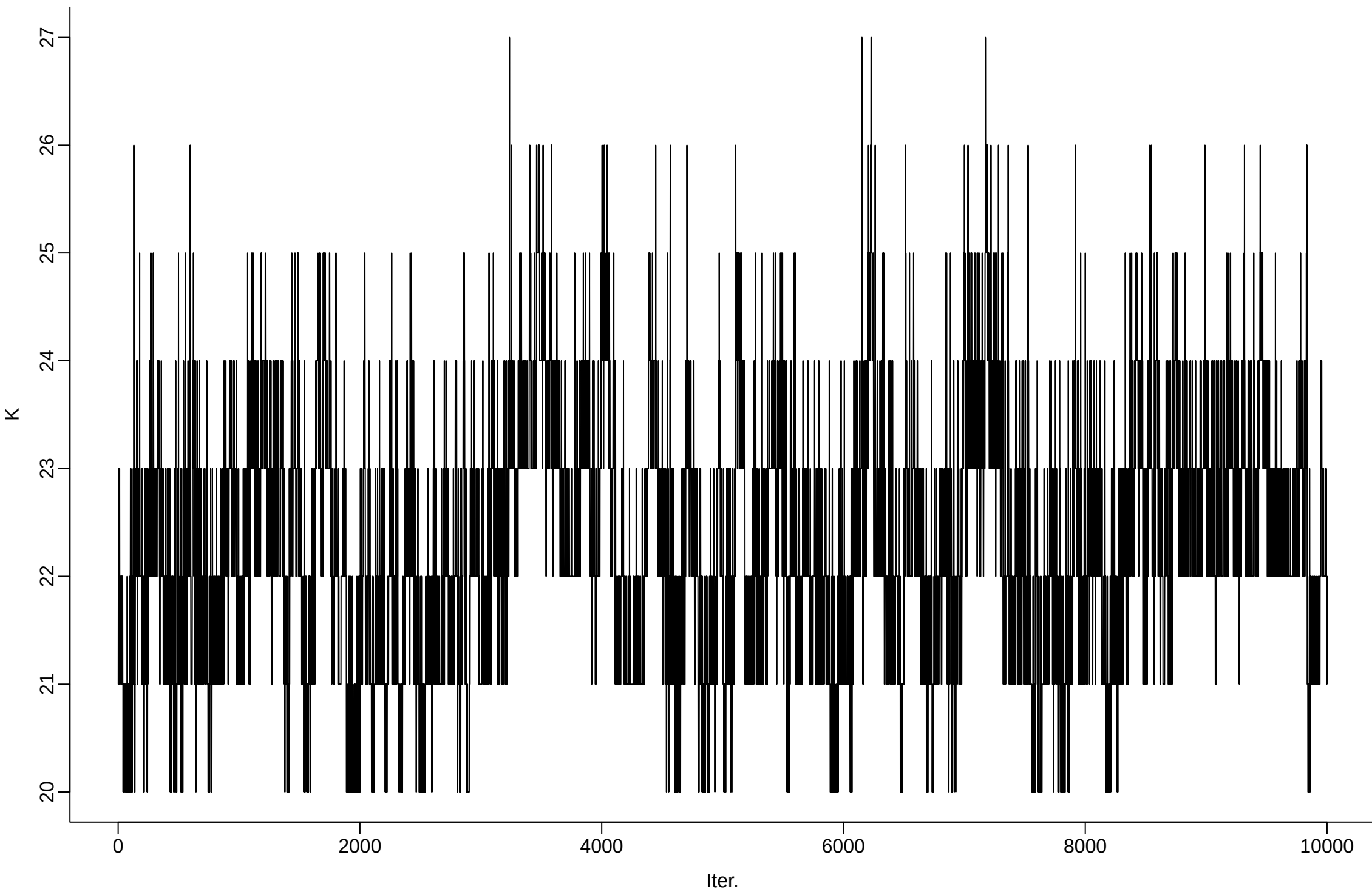
cfg264_r10_delta_1em02_beta0_1em02_gamma0_1em02_sigma0_7p5em01 | Total number of distinct topics
