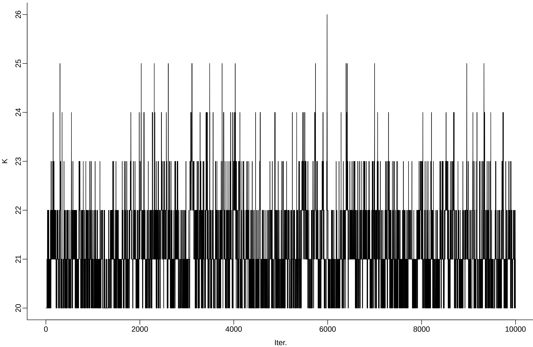
cfg336_r10_delta_1em02_beta0_1em03_gamma0_1em02_sigma0_9em01 | Total number of distinct topics
