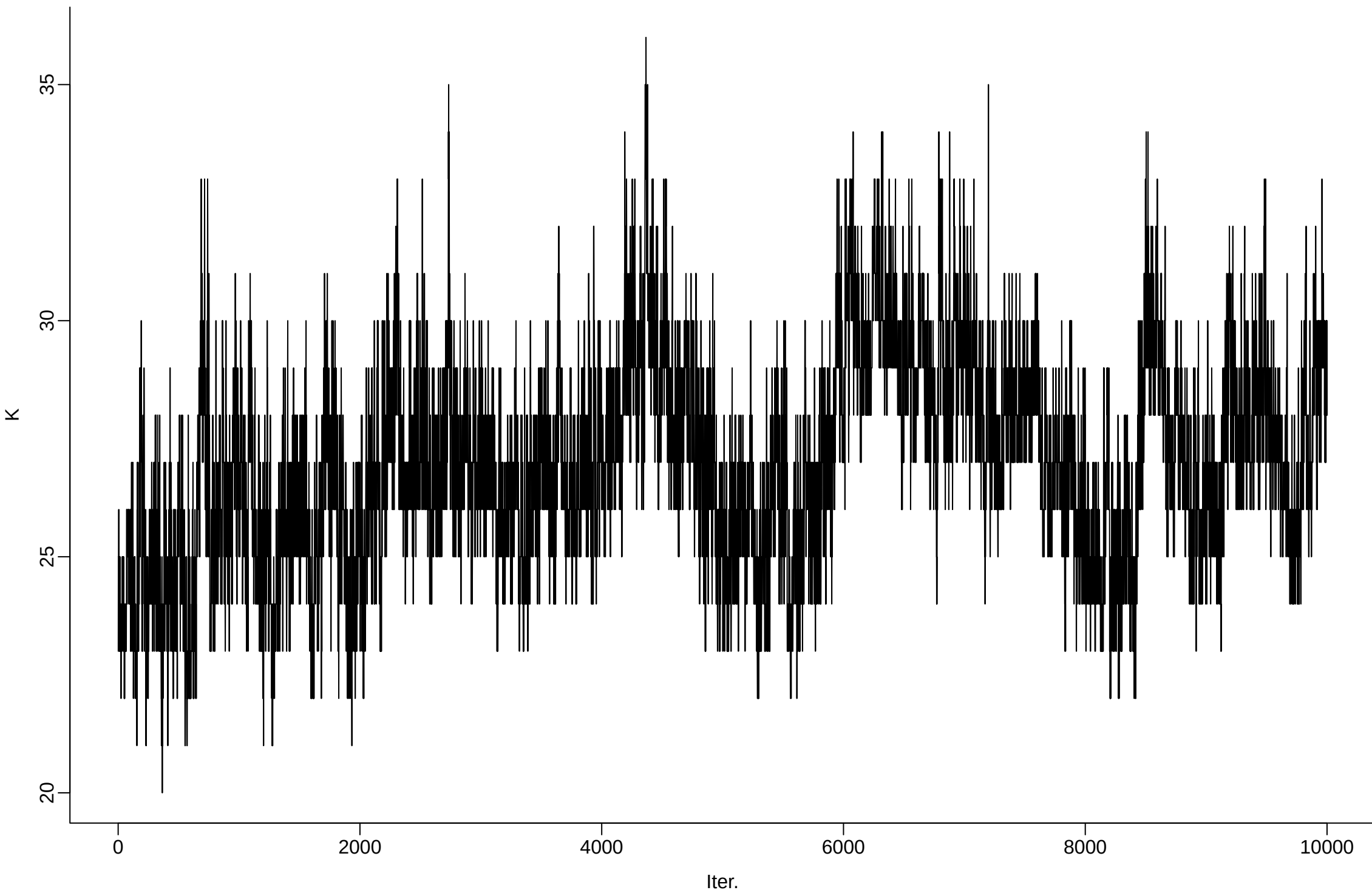
cfg353_r10_delta_1em03_beta0_1em02_gamma0_1em01_sigma0_9em01 | Total number of distinct topics
