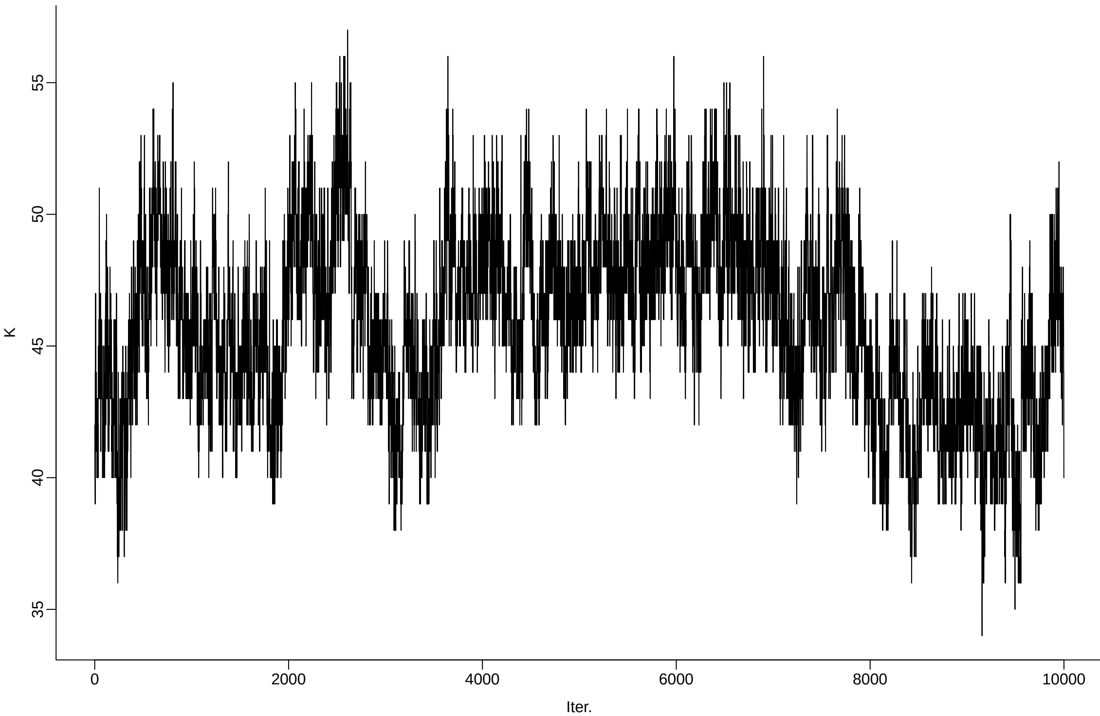
cfg359_r10_delta_1em03_beta0_1e00_gamma0_1em01_sigma0_9em01 | Total number of distinct topics
