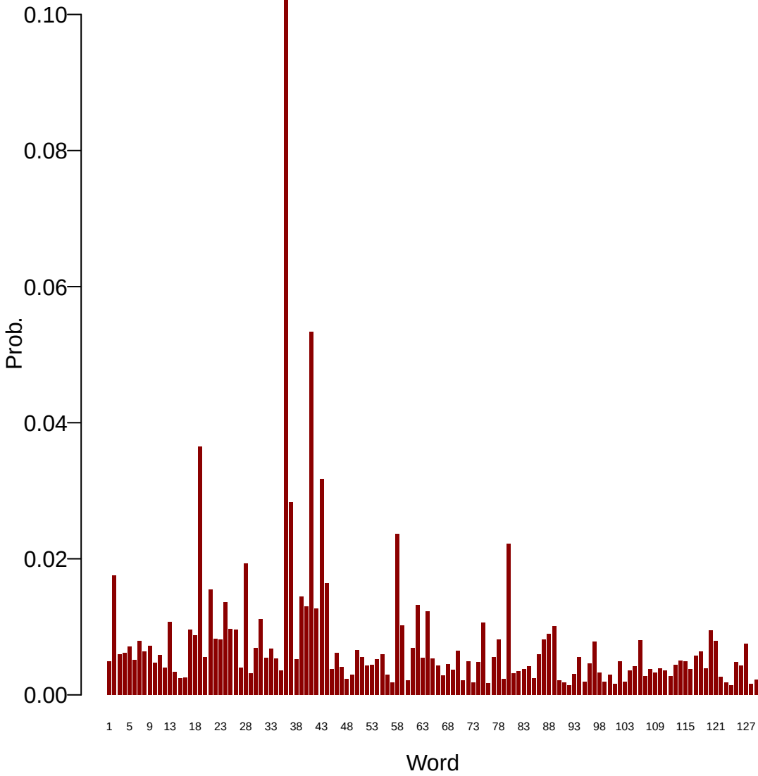
Topic: 13
