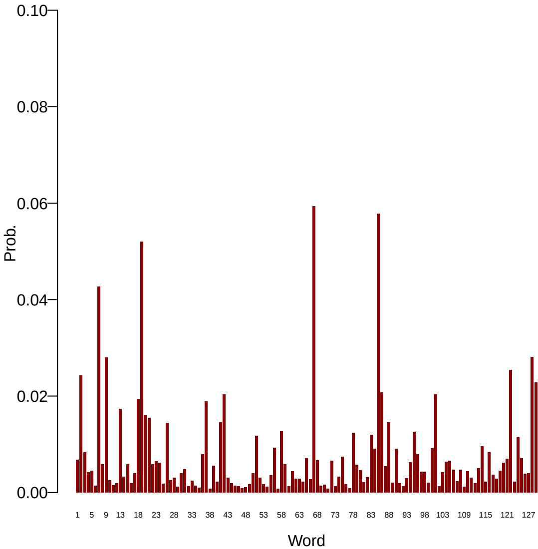
Topic: 20
