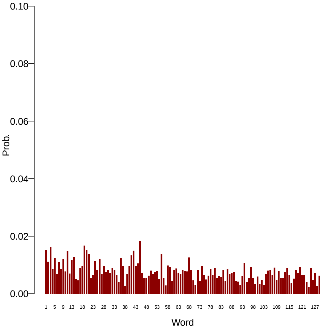
Topic: 8
