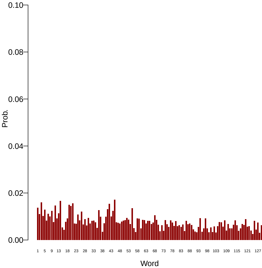
Topic: 27
