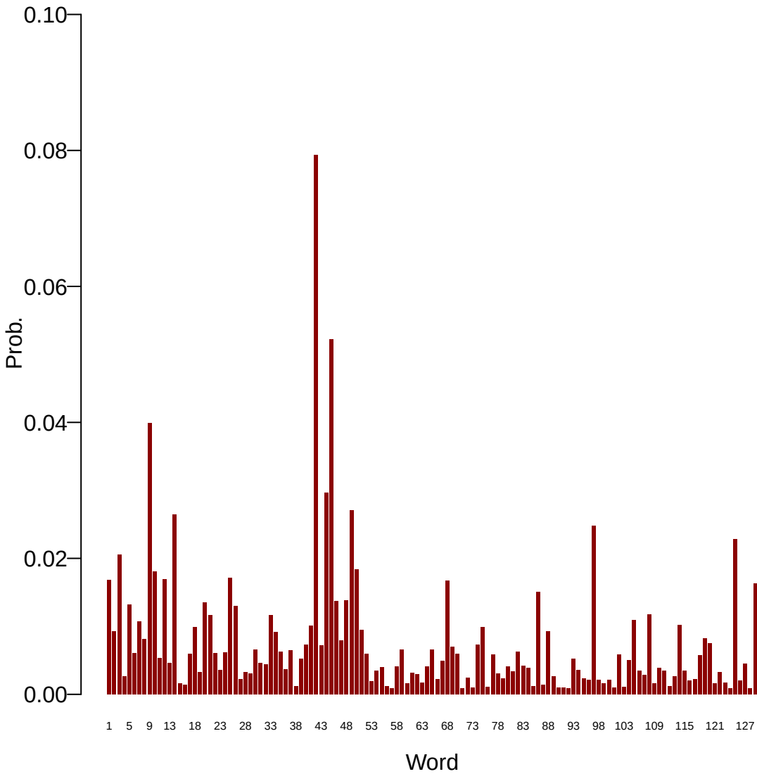
Topic: 28
