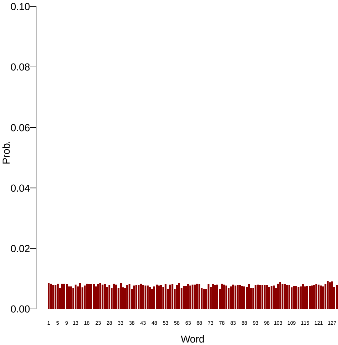
Topic: 40
