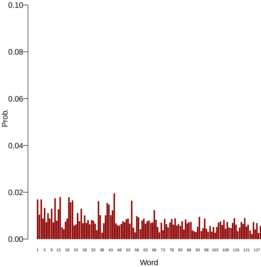
Topic: 39
