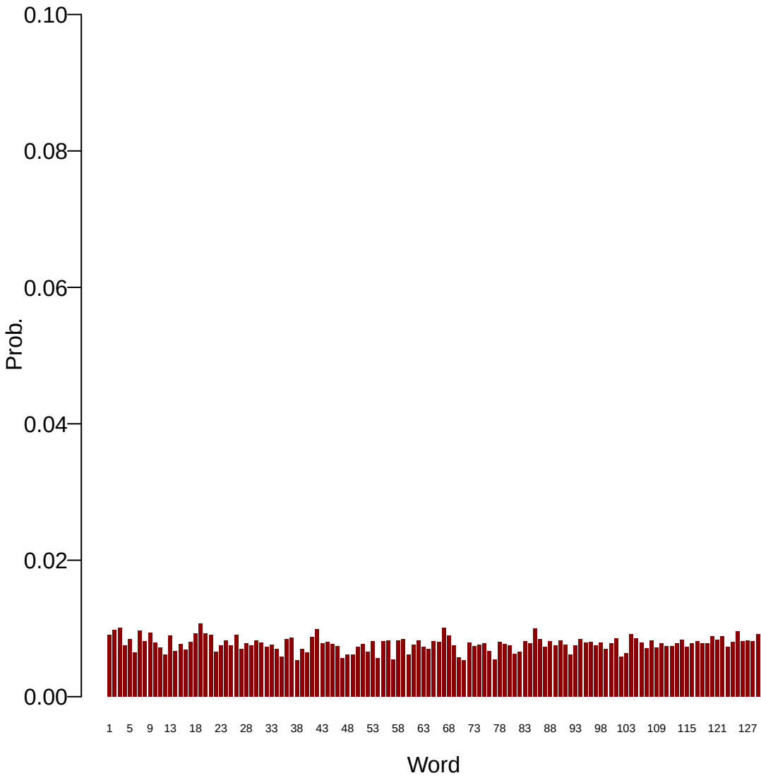
Topic: 38
