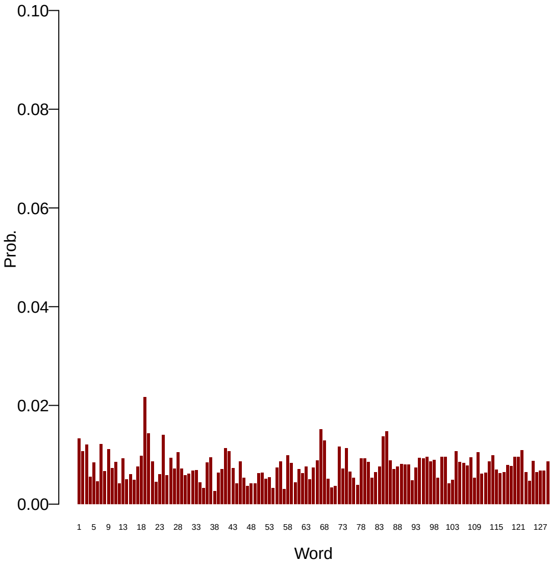
Topic: 19
