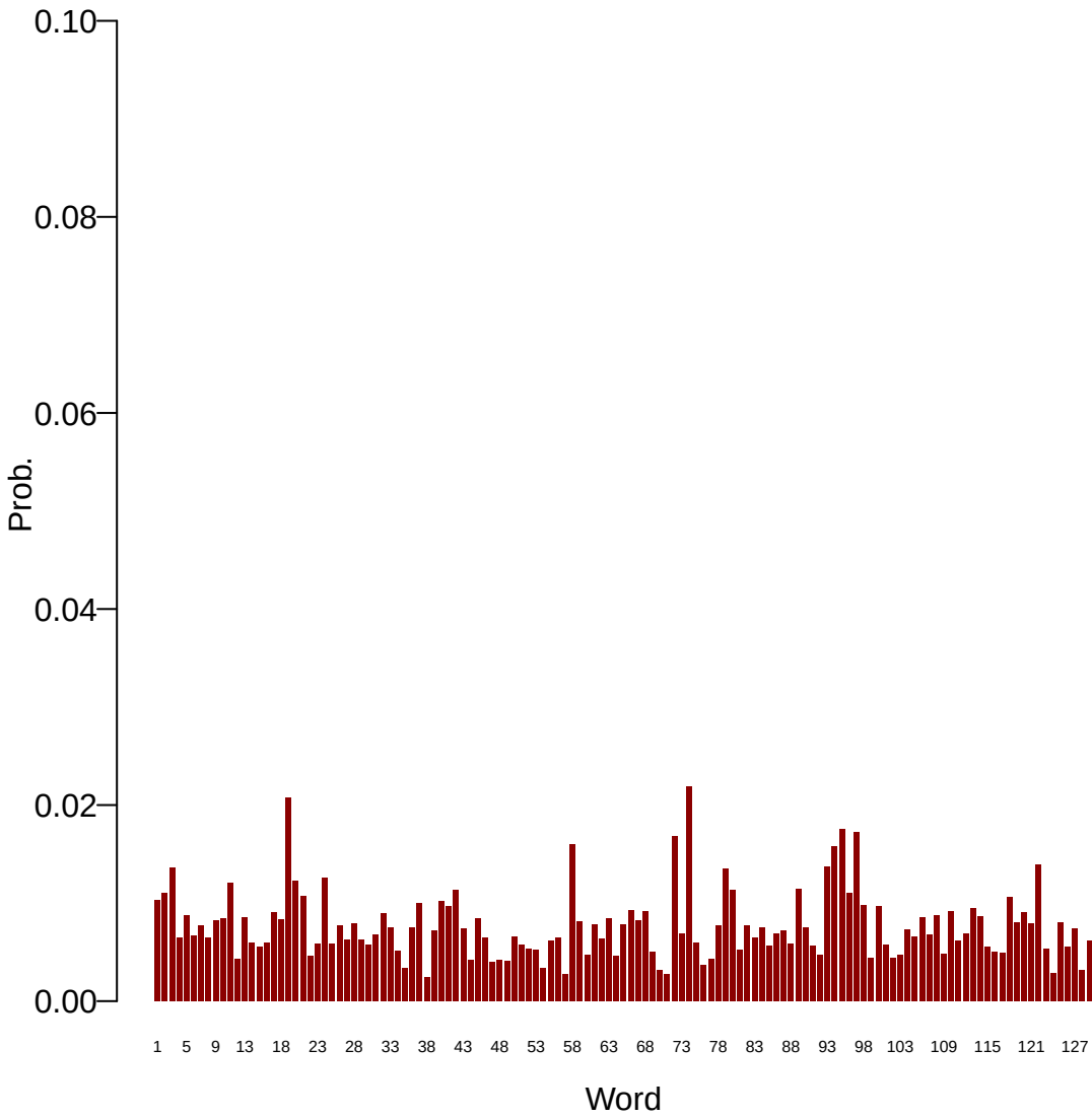
Topic: 33
