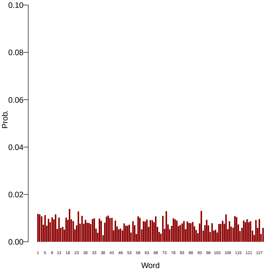
Topic: 9
