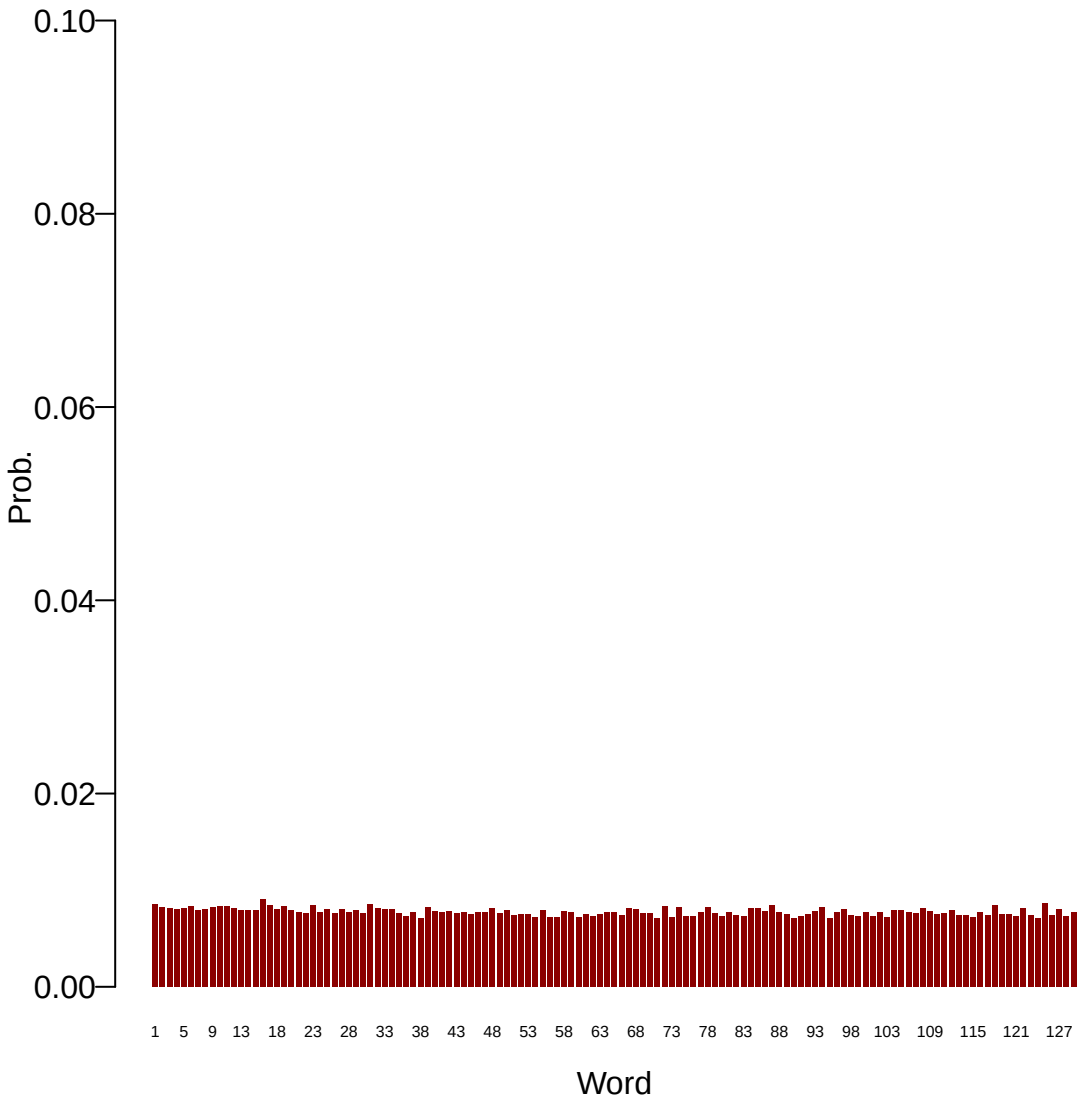
Topic: 17
