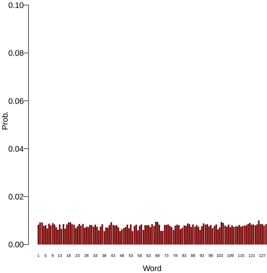
Topic: 41
