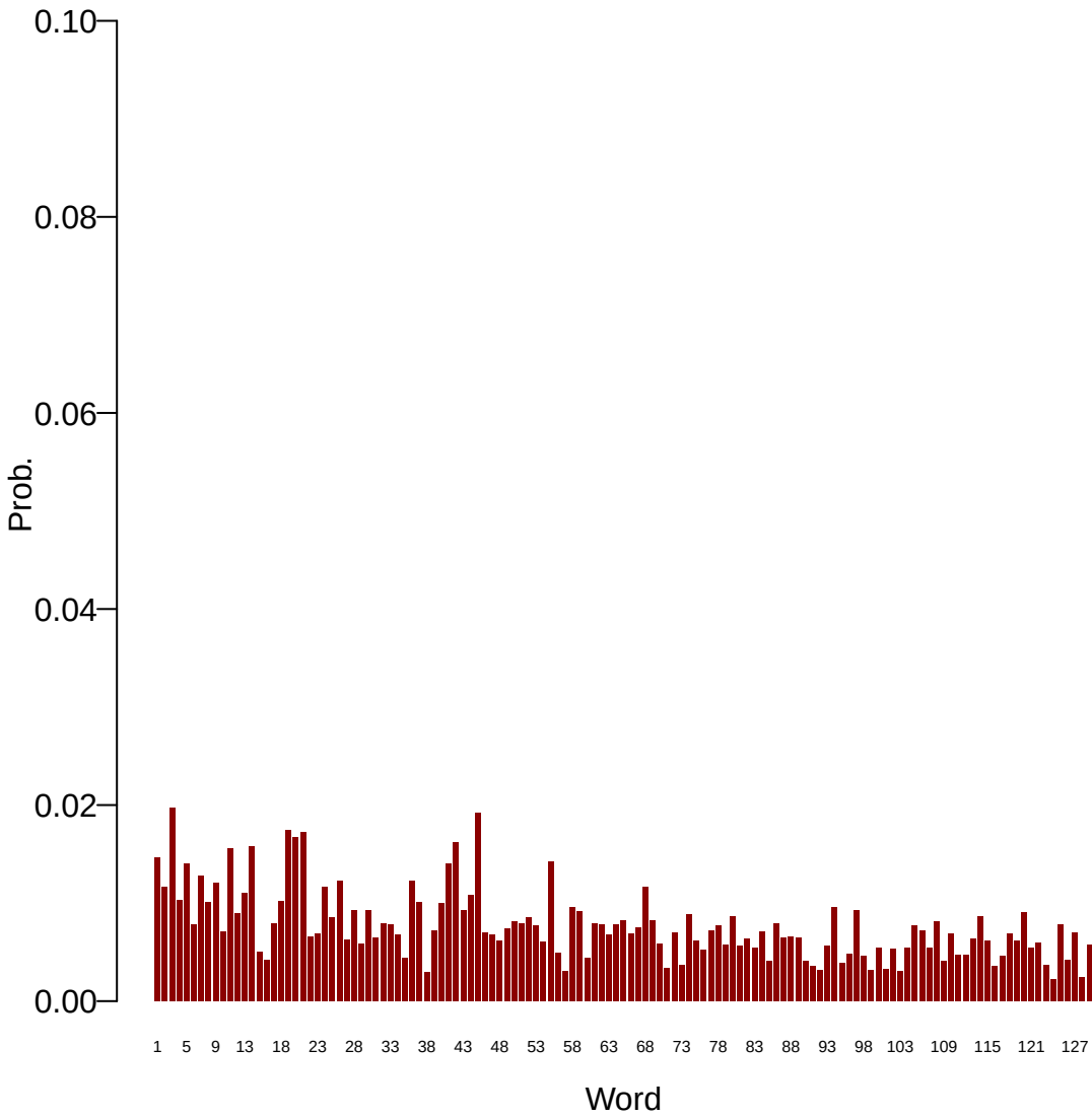
Topic: 21
