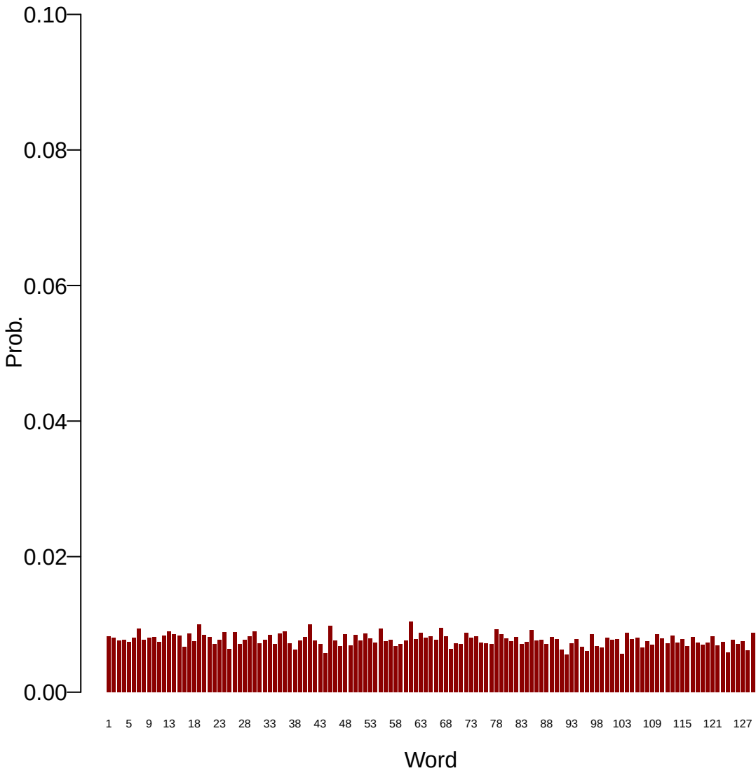
Topic: 42
