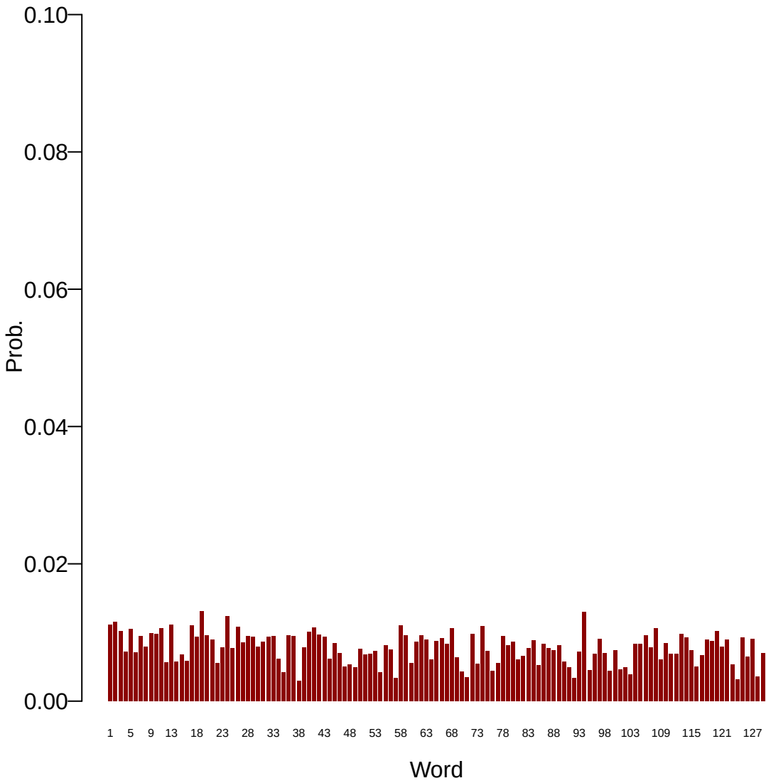
Topic: 5
