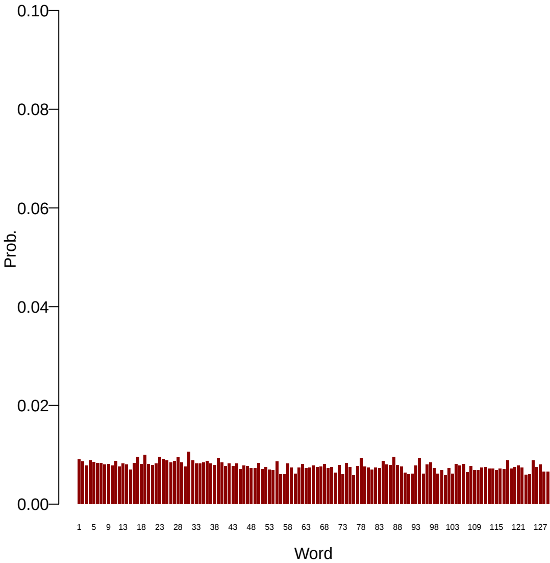
Topic: 36
