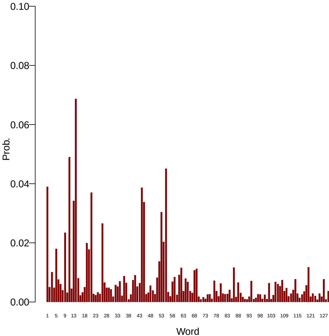
Topic: 31
