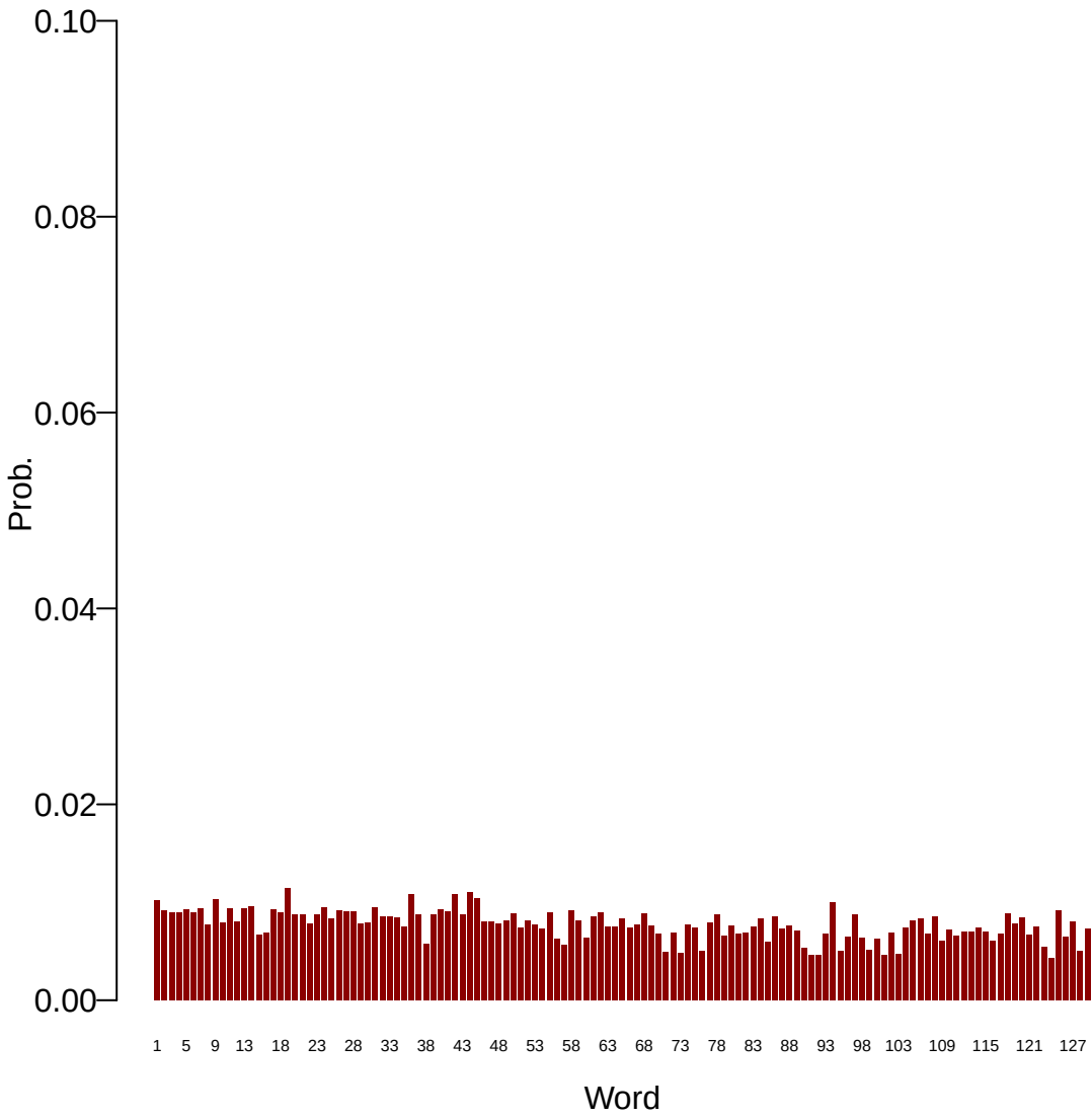
Topic: 26
