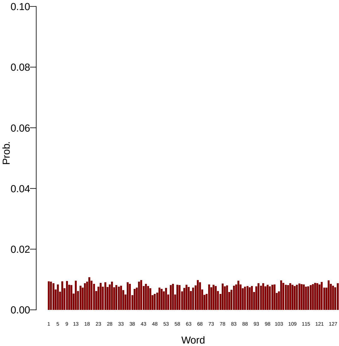
Topic: 29
