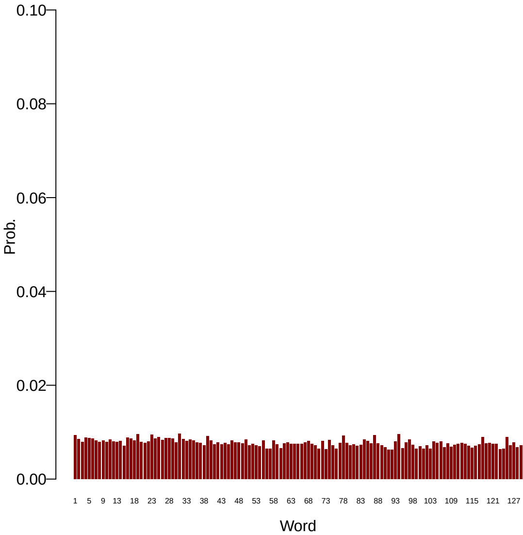
Topic: 22
