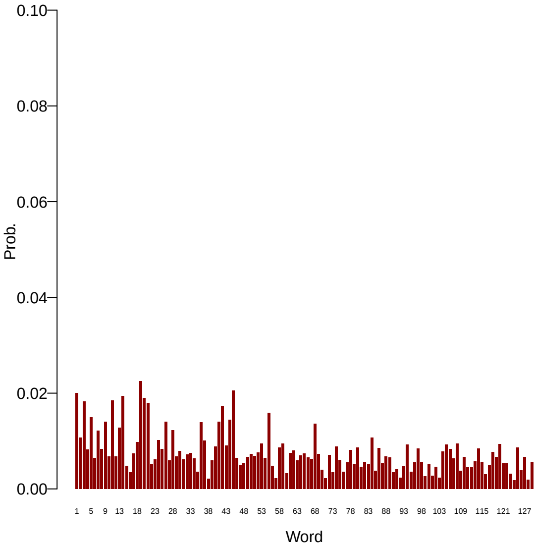
Topic: 3
