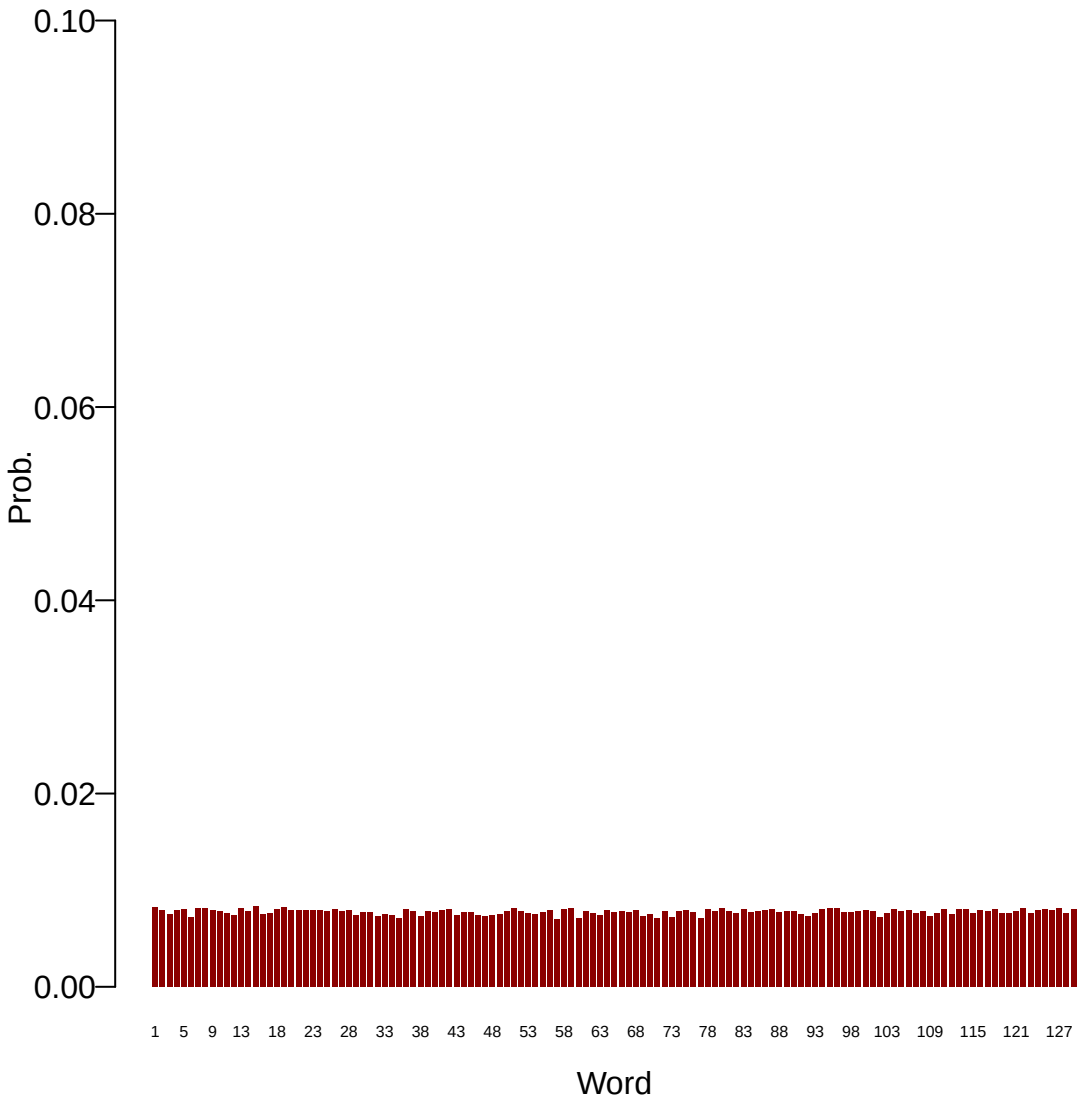
Topic: 34
