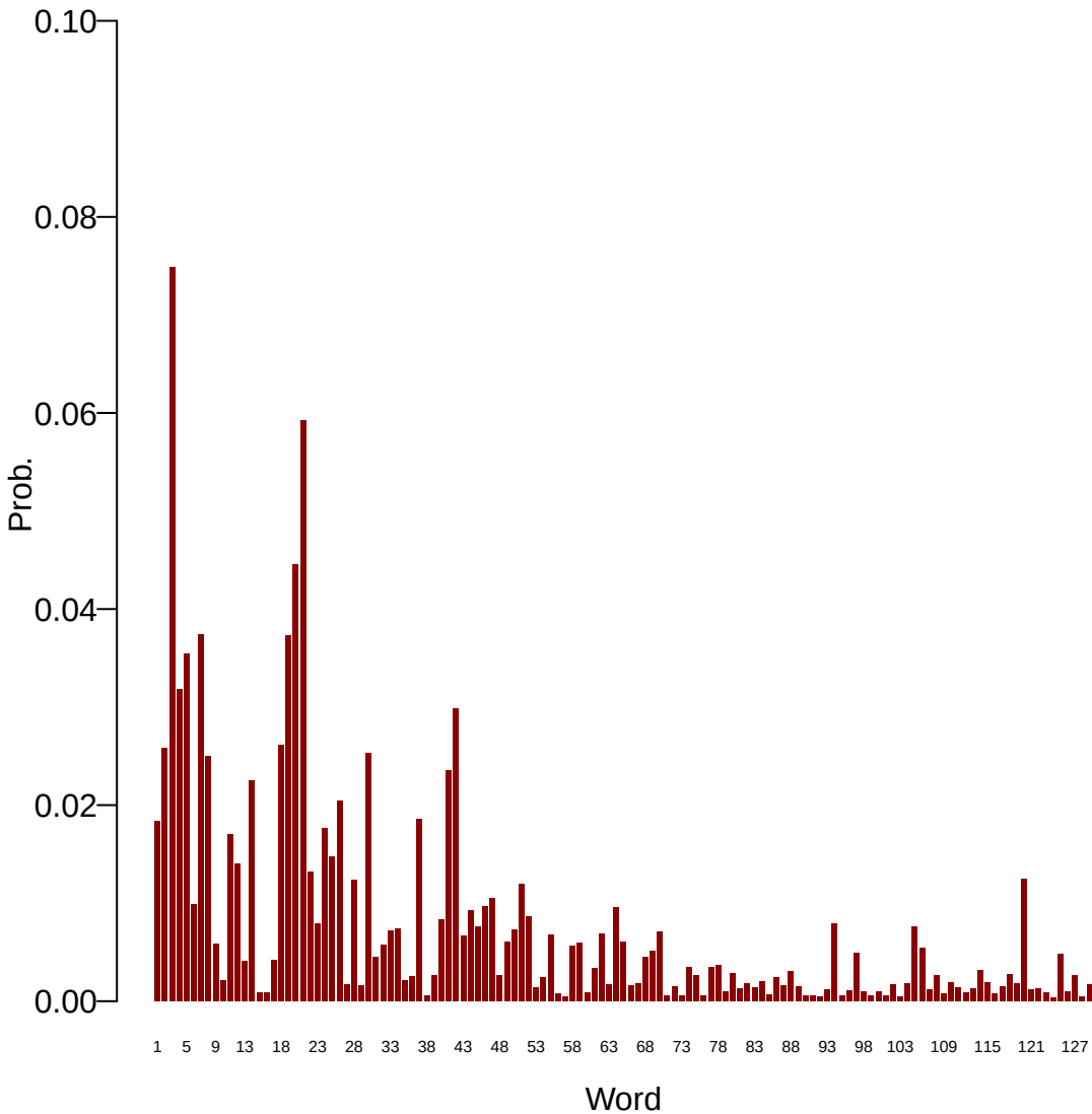
Topic: 11
