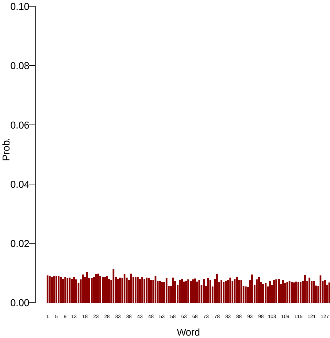
Topic: 24
