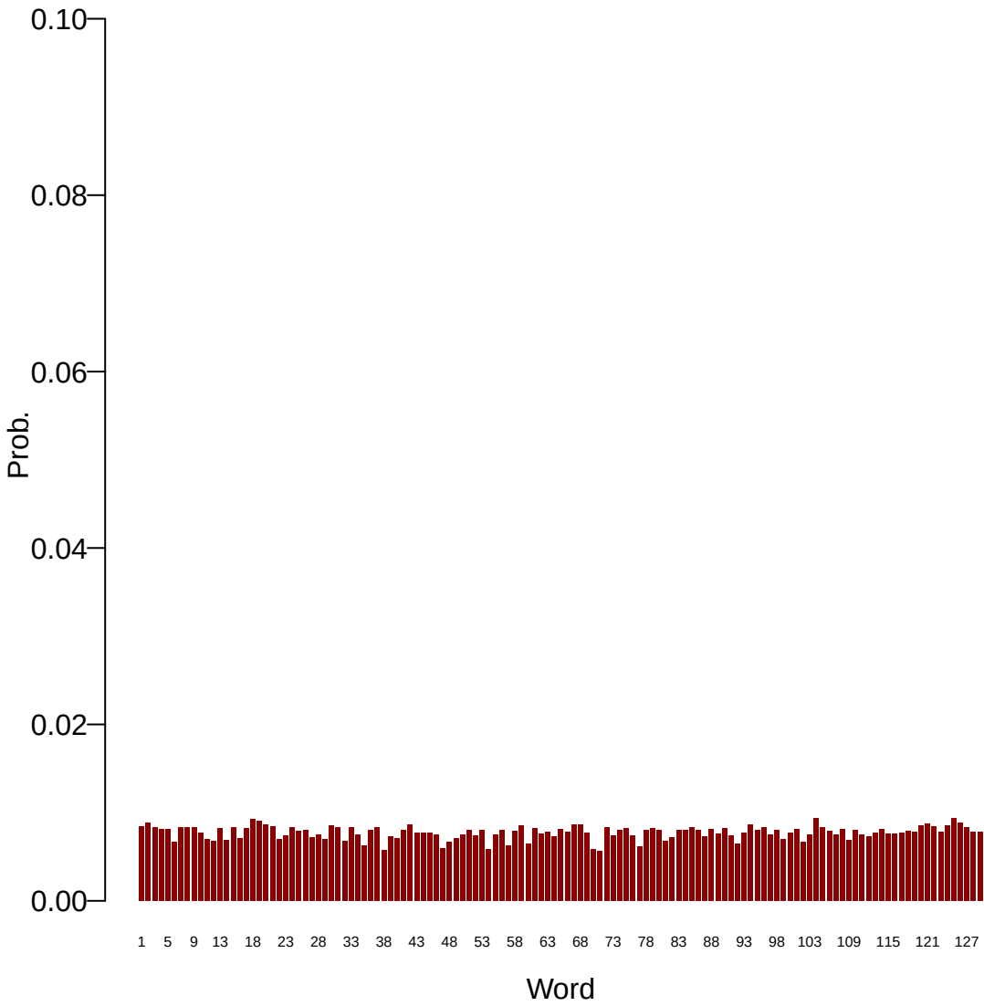
Topic: 35
