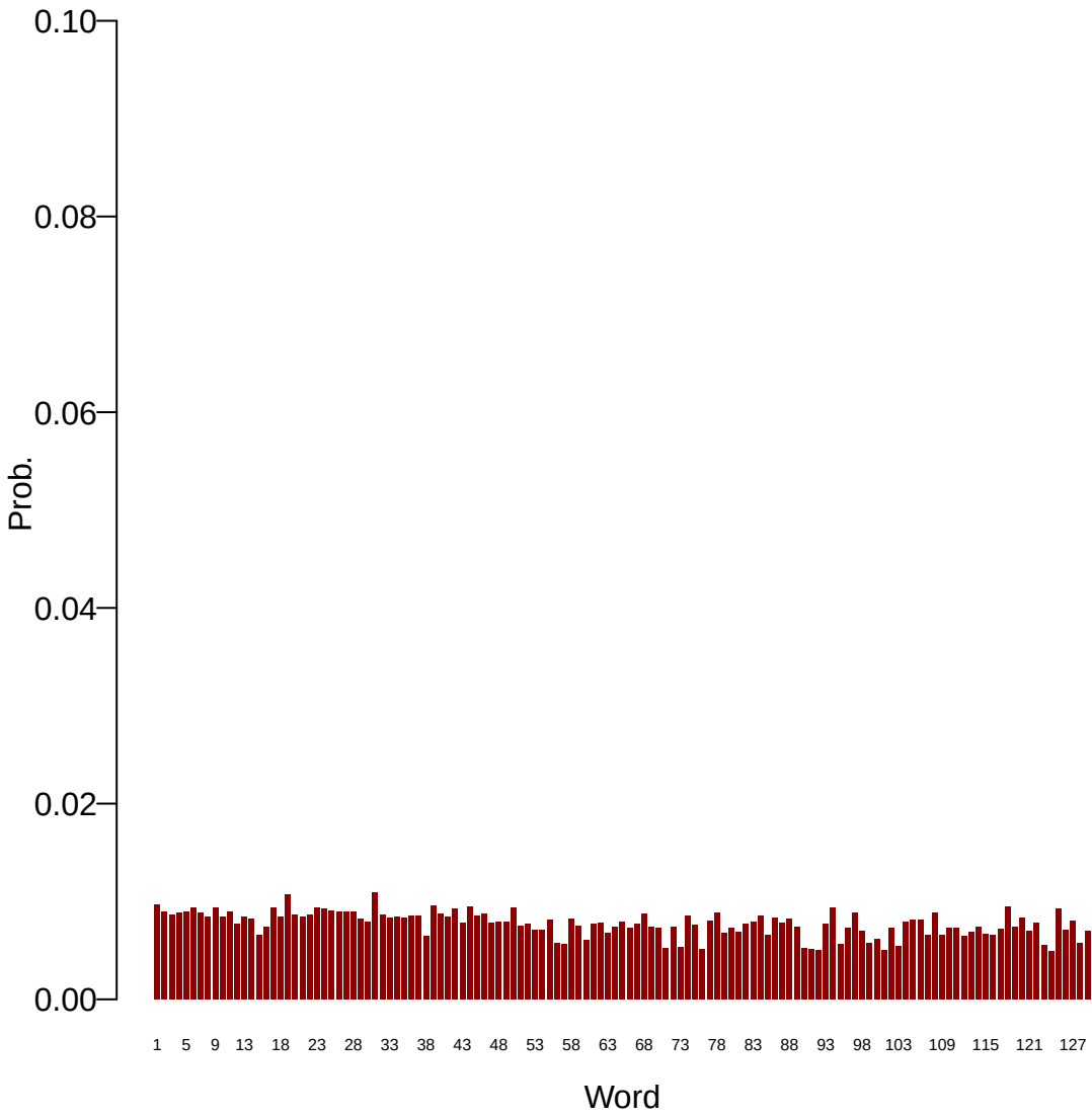
Topic: 18
