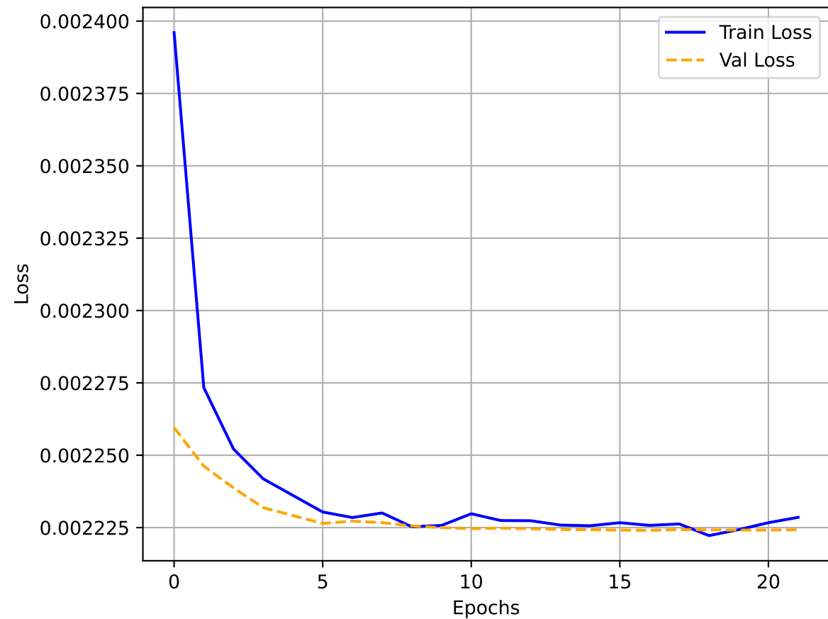
Loss function
