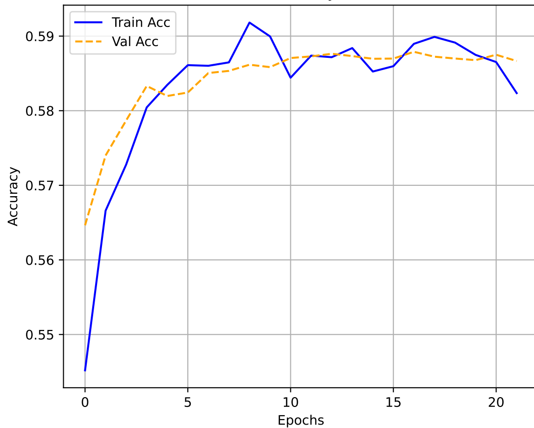
Accuracy
