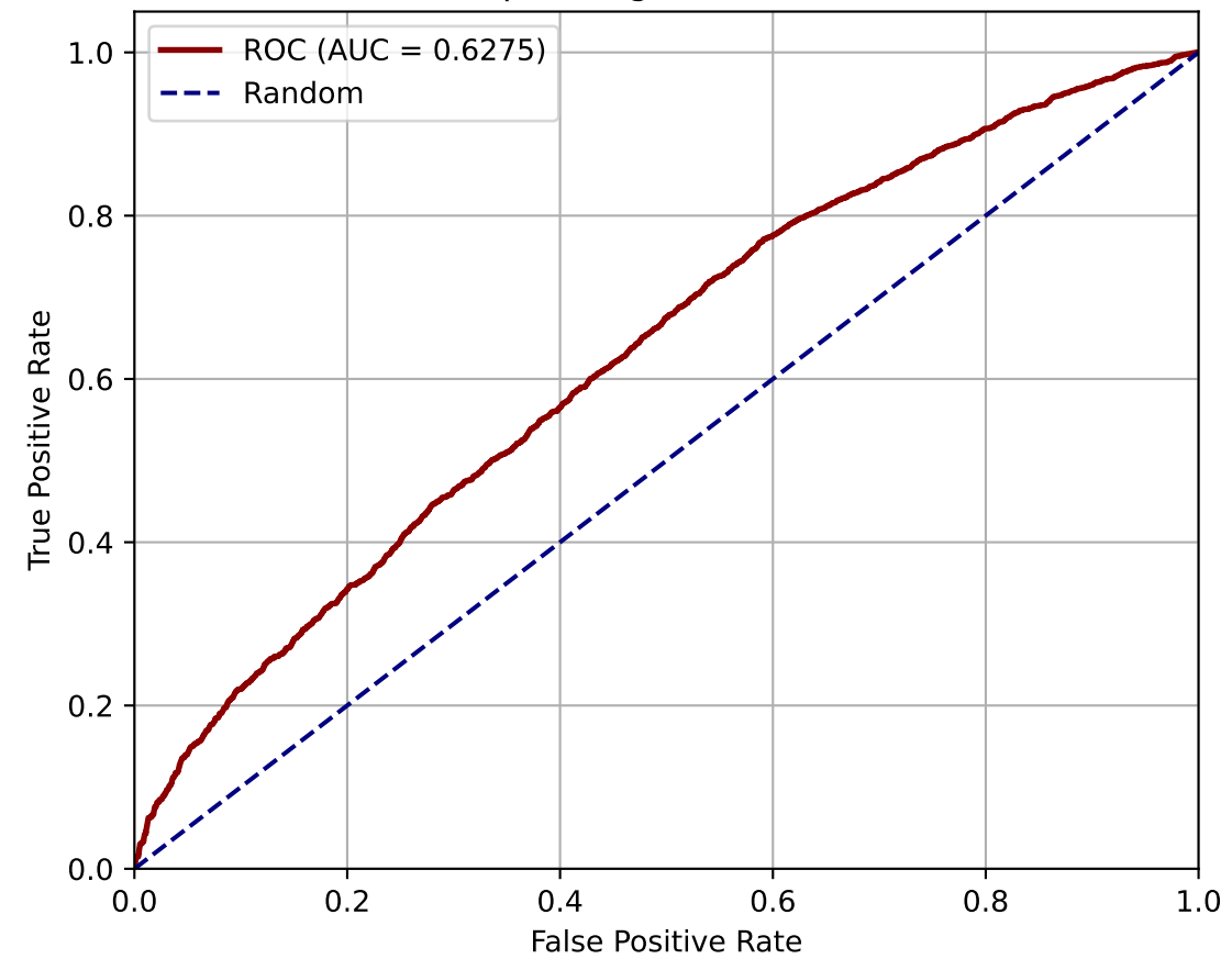
Receiver Operating Characteristic (ROC)
