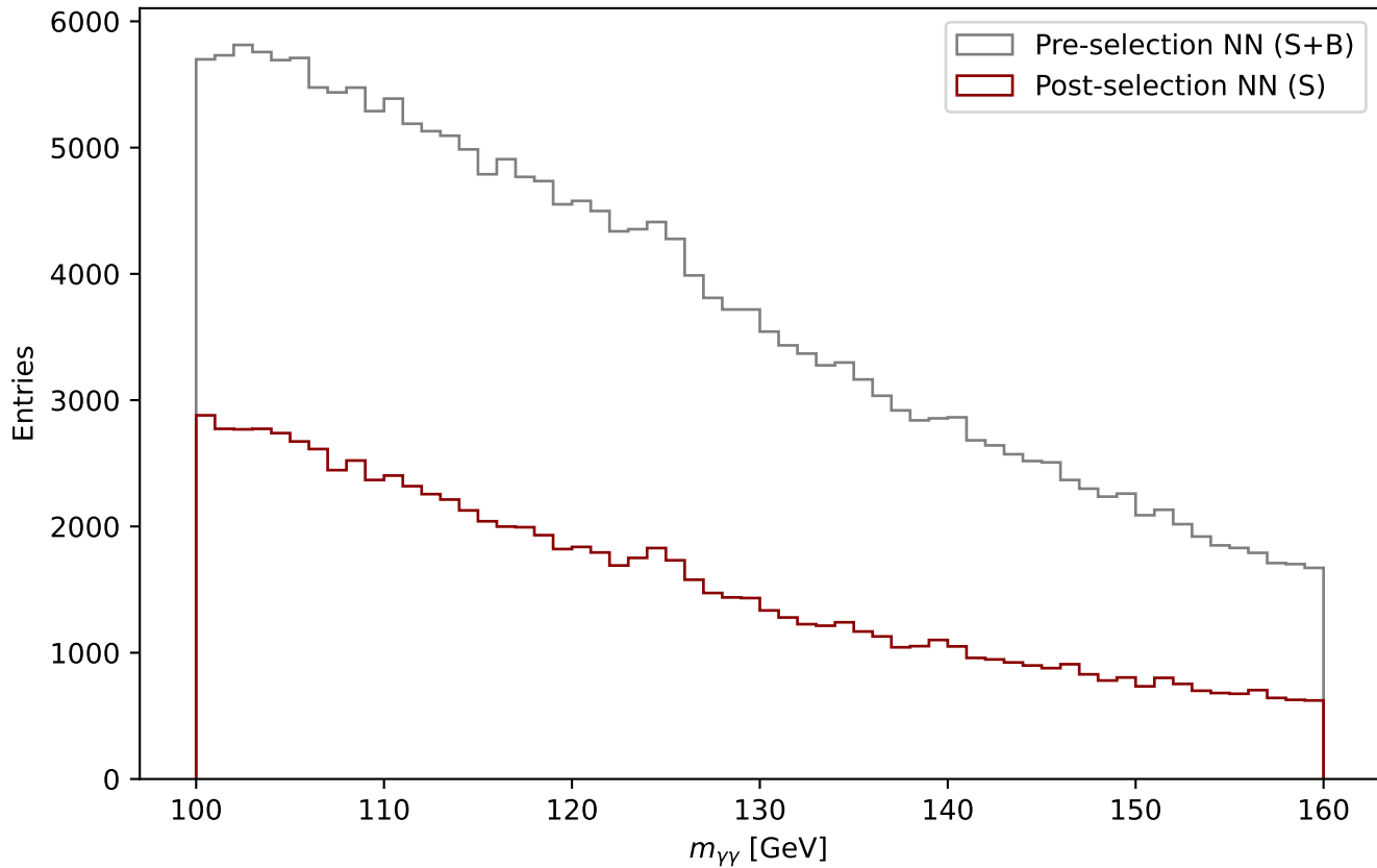
Diphoton invariant mass m_{\gamma\gamma} spectrum
