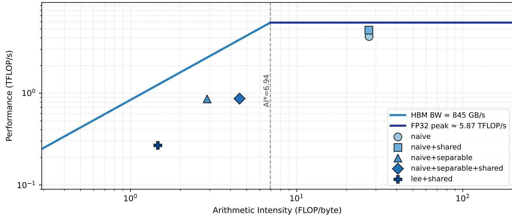
Roofline (FP32) with 5 DCT Kernels
