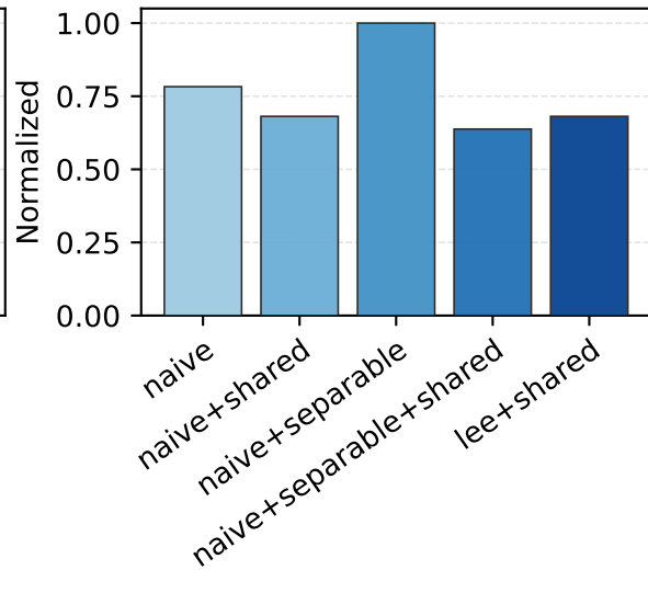
GPU normalized
