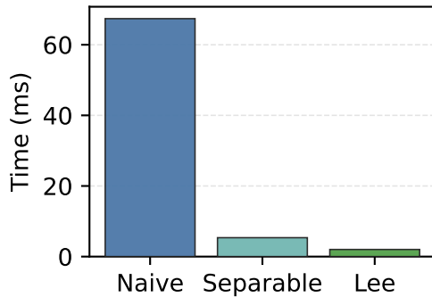
CPU normalized (-O3)
