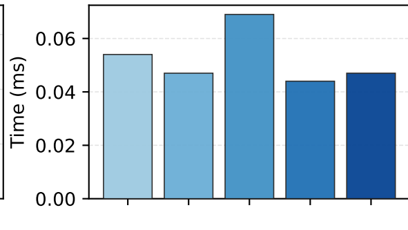
GPU normalized
