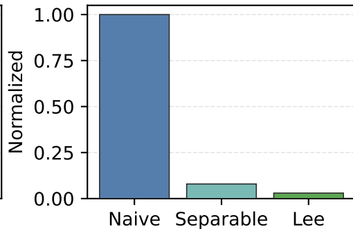
CPU normalized (-O3)
