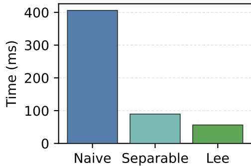
CPU normalized (no -O3)
