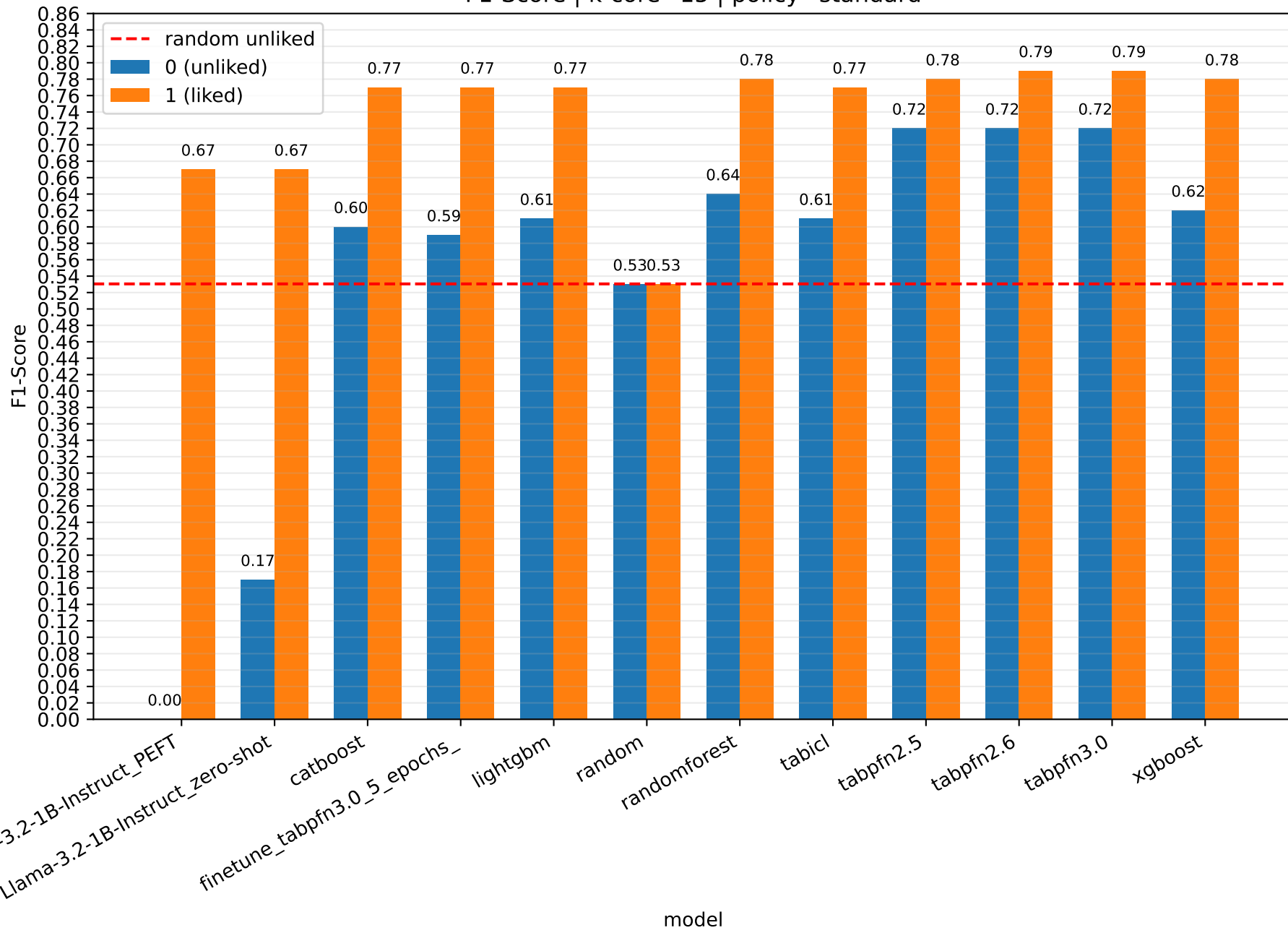
F1-Score | k-core=15 | policy=standard
