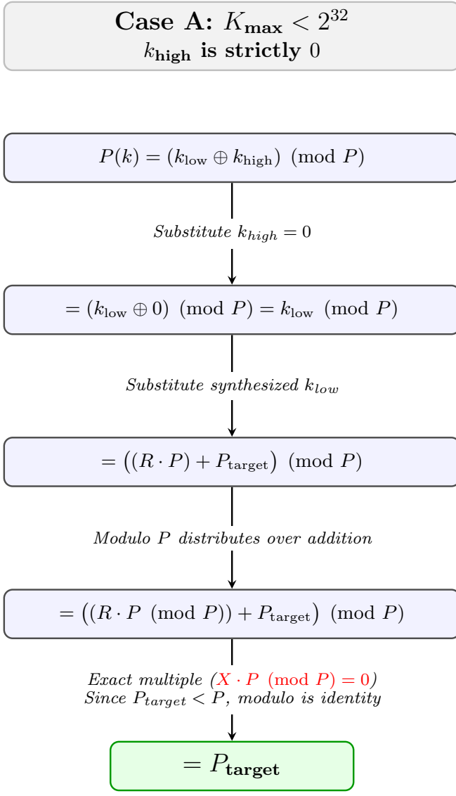
Figure 3: Mathematical derivation proving deterministic routing to P_{\text{target}} , adapting based on the bounds of K_{\max} . pgfplots
