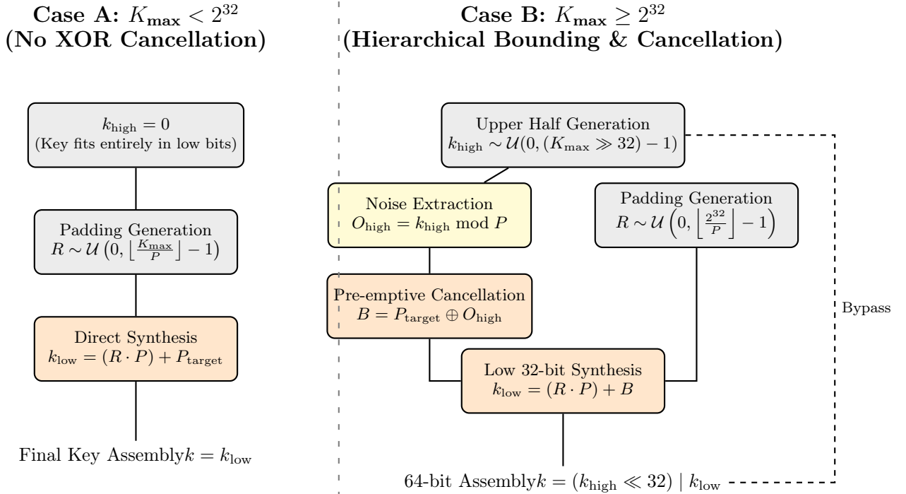
Figure 2: Key synthesis pipeline conditionally branching based on the global maximum key limit ( K_{\text{max}} ).
