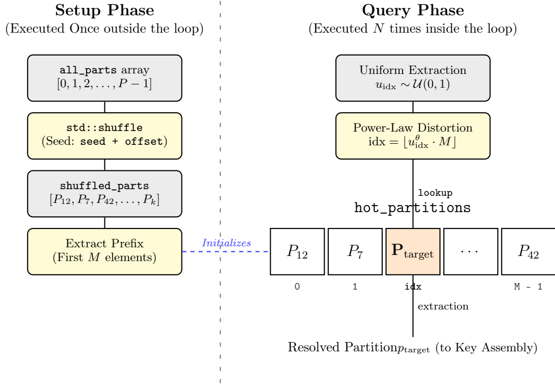
Figure 1: Lifecycle of the sparse partition subset. The hot_partitions array is populated once by shuffling the full partition space and extracting M elements. During generation, a power-law distortion with shape parameter \theta is applied to a uniform random variable, skewing the index lookup towards the hottest partitions to resolve the physical ID ( P_{\text{target}} ).
