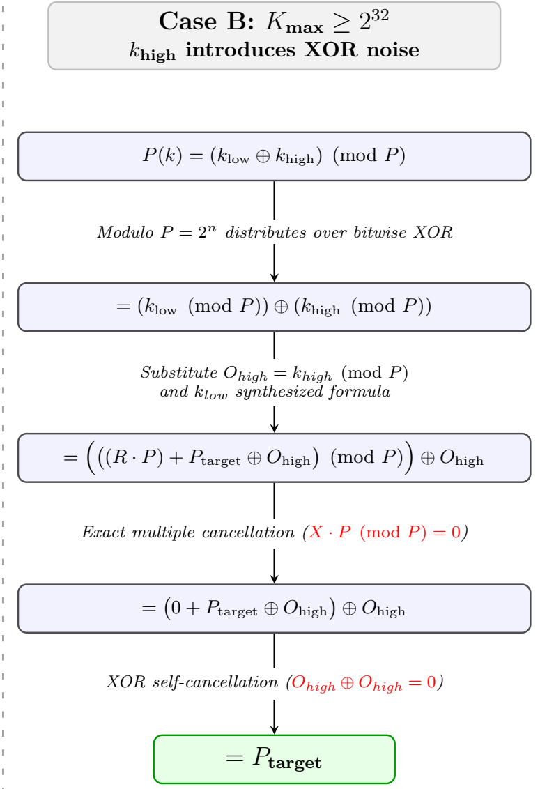
Figure 3: Mathematical derivation proving deterministic routing to P_{\text{target}} , adapting based on the bounds of K_{\max} . pgfplots
