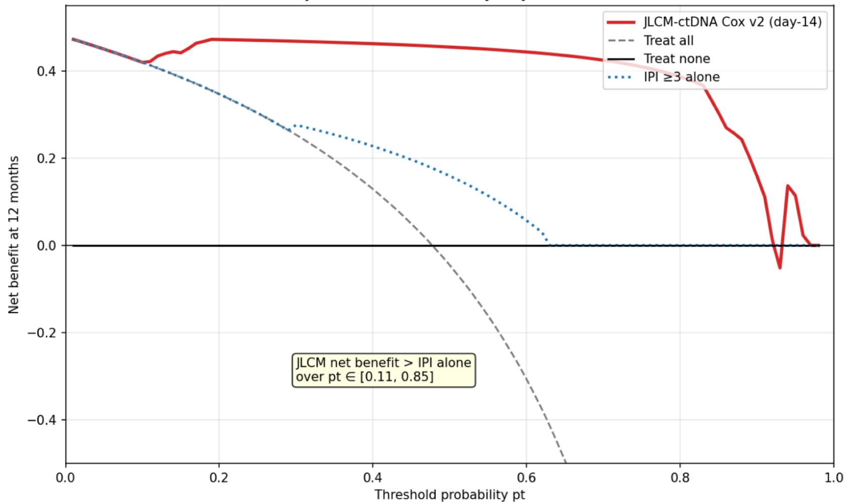
Decision curve analysis — net benefit of day-14 JLCM-ctDNA vs IPI vs all/none
