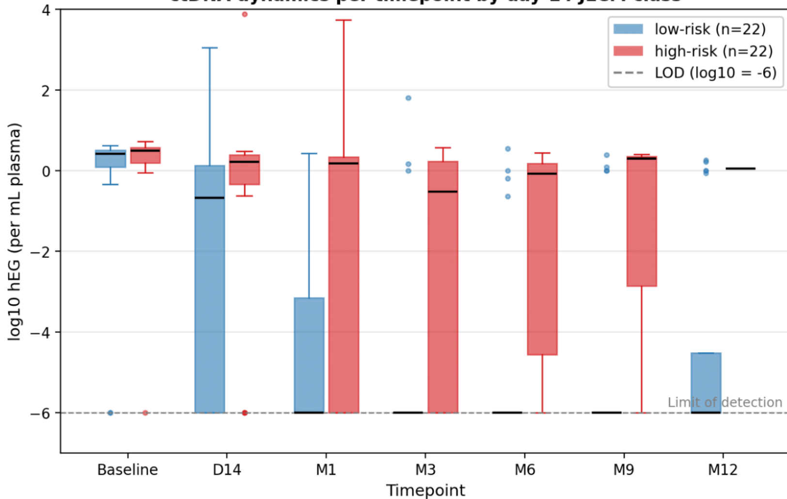
ctDNA dynamics per timepoint by day-14 JLCM class
