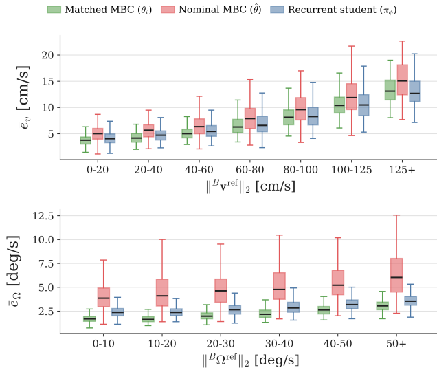
Fig. 5. Closed-loop velocity-tracking performance of the nominal MBC, matched teacher, and recurrent student. The plots show the distributions of mean linear and angular tracking errors across the test set.
