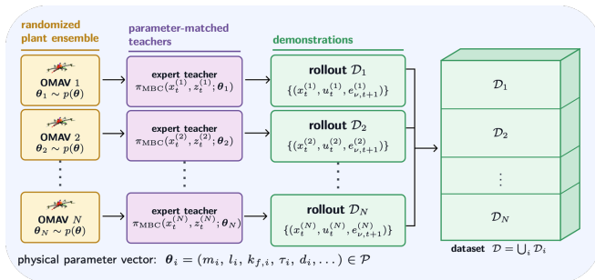
Fig. 3. Parameter-matched model-based controllers generate demonstrations for randomized OMAV plants.
