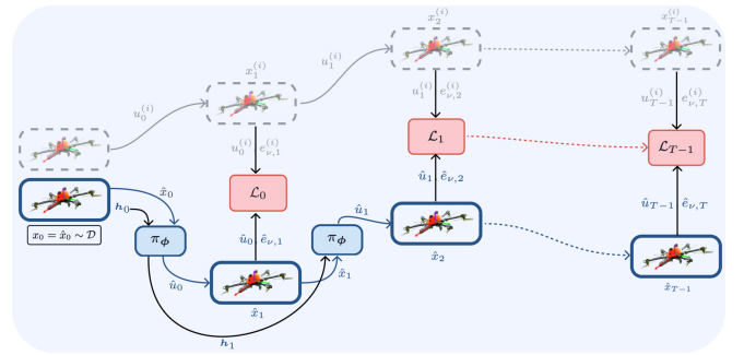
Fig. 4. During training, the recurrent student is unrolled in closed loop through the corresponding differentiable plant dynamics, and each step is supervised by both teacher-command imitation and velocity-tracking behavior matching.
