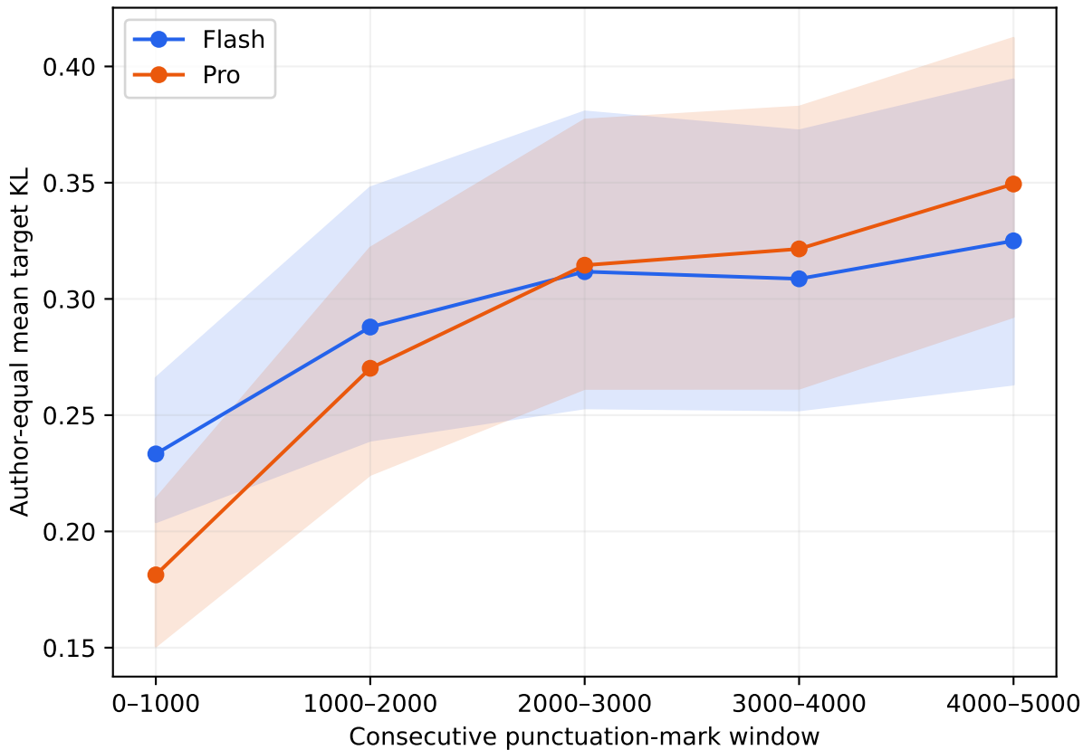
Both models drift away from target punctuation profiles
