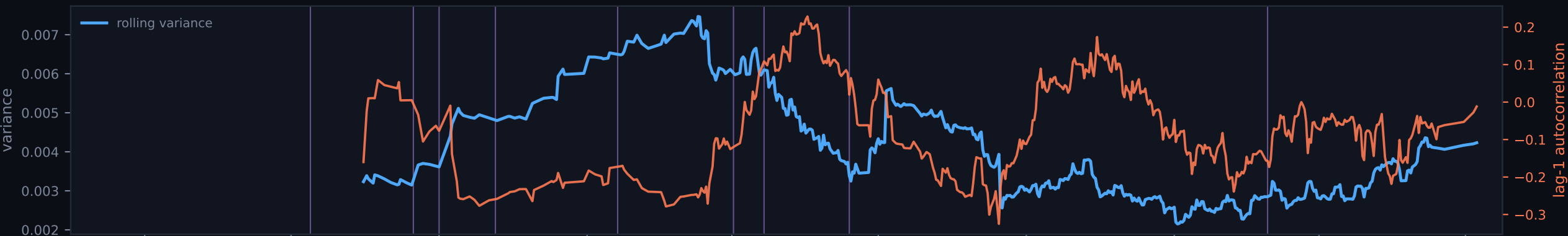
volatility diagnostic: variance and lag-1 autocorrelation of the daily nightmare-index residual
