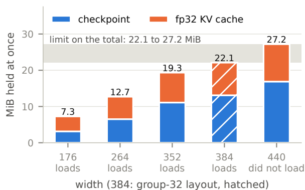
Figure 4: Checkpoint and fp32 KV cache per width (six layers, context 512), and whether the model loaded. The shaded band is where the limit on the two-block total must lie; width 384 is a group-32 layout. The largest single block directly after a reset was 21.53 MiB.
