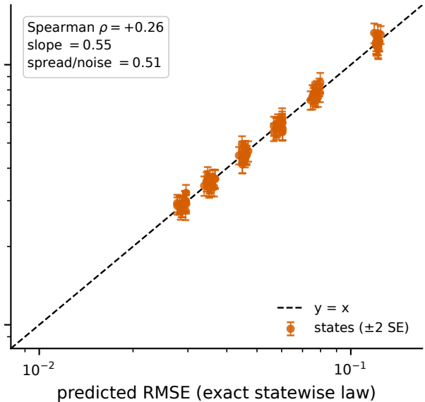
fixed estimand (noisy-pure, control)
