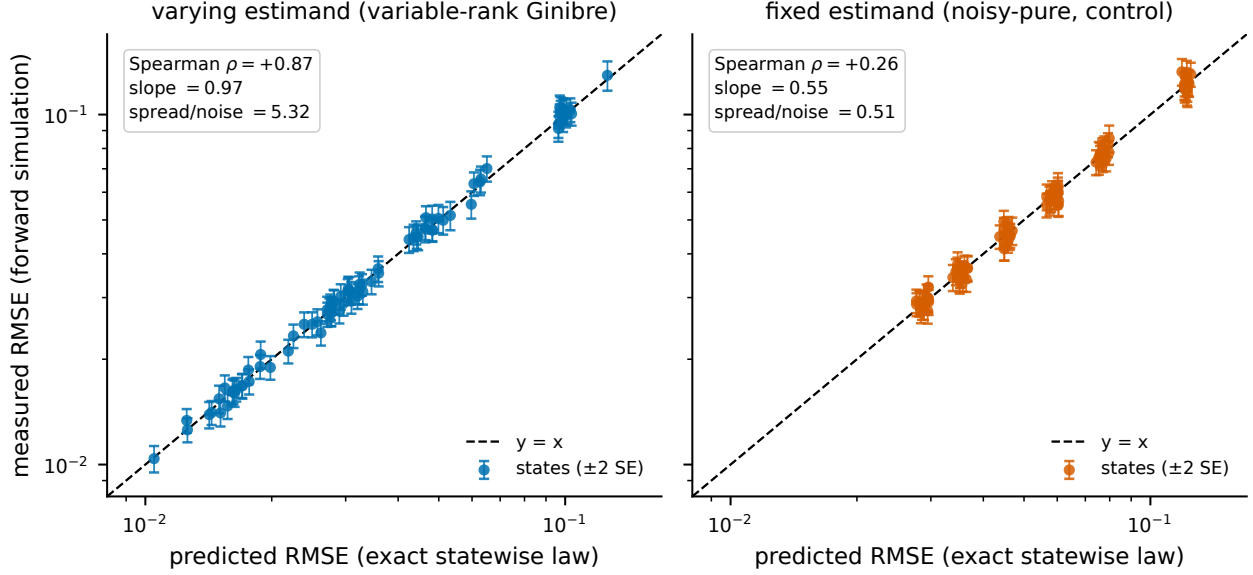
FIG. 3. Statewise validation. Predicted versus measured single-copy RMSE for individual states at k = 2 , n = 3, 4, 5 and two budgets, 14 states per cell, 300 trials each. Predictions come from each state's exact \zeta_1, \zeta_2 , with nothing fitted to the plotted points. Left: a varying-estimand family, where the statewise threshold spans an order of magnitude, so the law is tested state by state. Right: the fixed-estimand noisy-pure family as a negative control; its statewise spread is below the measurement noise, so no ordering can be resolved and a family-average law would score the same. Both panels share one scale.
