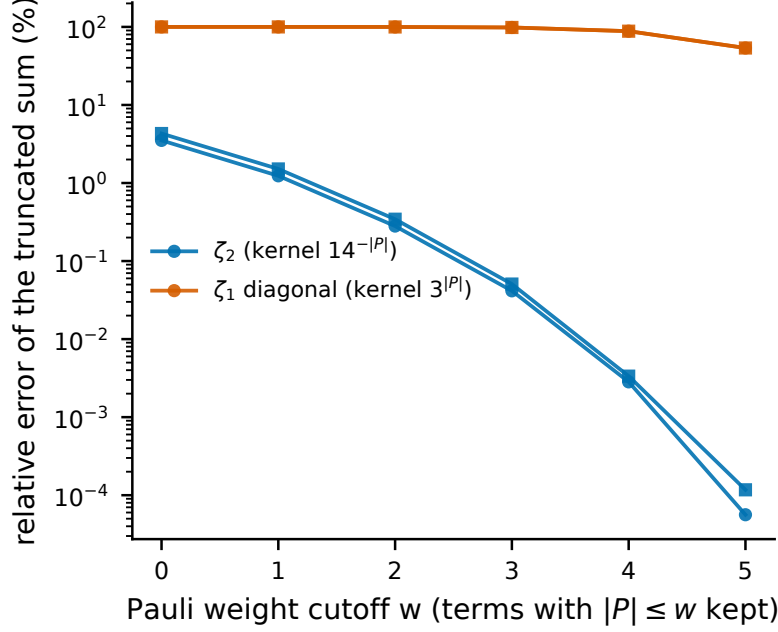
FIG. 1. The two projection variances read opposite ends of the Pauli spectrum. Relative error of each functional when its sum over Pauli strings is truncated to weight |P| \leq w , at n = 6 (circles noisy-pure, squares Haar-pure). \zeta_2 carries the kernel 14^{-|P|} , which suppresses high weight, so a few percent of the strings determine it. The \zeta_1 diagonal carries 3^{|P|} , which amplifies high weight, so most of the spectrum is needed. The cutoff w = n is exact by construction and is not plotted.
