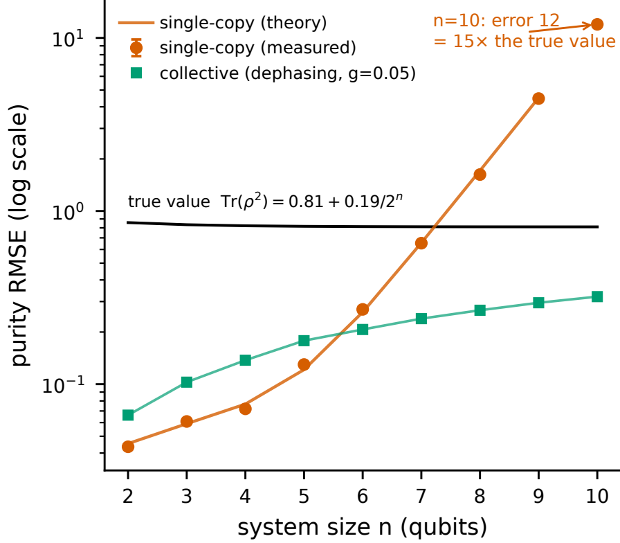
FIG. 8. Single-copy error growth against a bounded collective error. Single-copy purity RMSE for the unbiased U-statistic versus n out to n = 10 at a fixed copy budget of M = 2000 (log scale; measured points with 68% CIs, theory line with no parameters fitted to the crossover data; noisy-pure ensemble, collective route under dephasing at g = 0.05 ), with the exact per- n true purity \text{Tr}(\rho^2) = 0.81 + 0.19/2^n marked (0.858 at n = 2 , approaching 0.81). By n = 10 the single-copy error reaches \sim 12 while the collective error (green) stays bounded. Projecting the single-copy estimate into the physical range (Sec. 7.3) caps it at 0.582, but does not restore its usefulness: from n = 7 on it is beaten by a constant fixed at the midpoint of that range, which uses no data at all.
