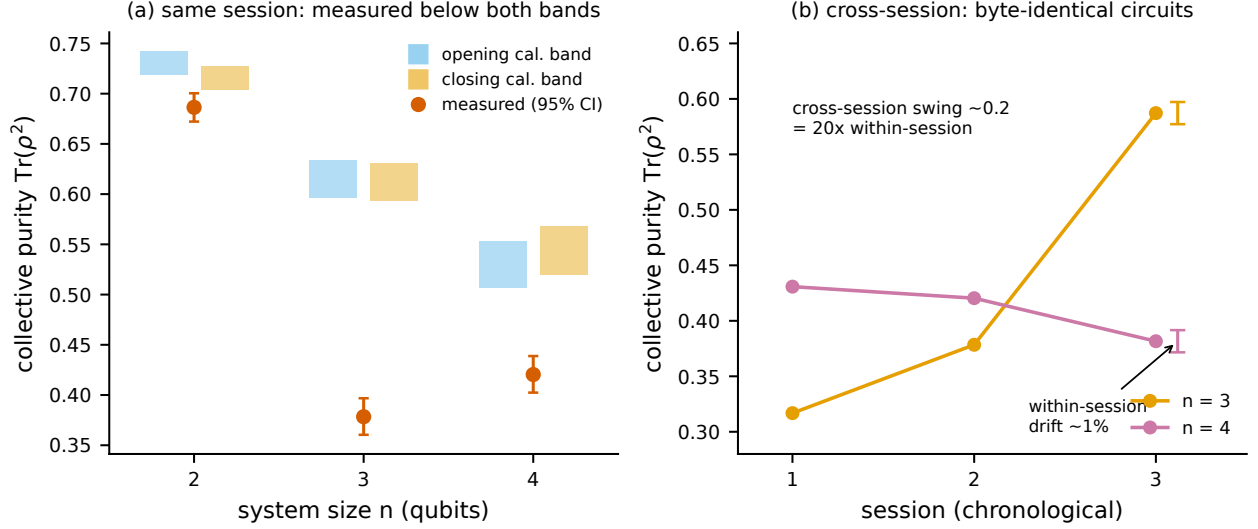
FIG. 6. Hardware: cross-session drift explains the gap. (a) Measured collective purity (vermillion, 95% CI) at n = 2, 3, 4 against the pre-registered same-session prediction bands from the opening (blue) and closing (orange) readout calibrations; every measurement falls below both bands. (b) The same byte-identical circuits across three sessions: the n = 3 register healed ( 0.32 \rightarrow 0.59 ) while n = 4 drifted down ( 0.43 \rightarrow 0.38 ), and the ordering flipped. Cross-session drift ( \sim 0.2 ) is about 20\times the within-session drift (scale bar).
