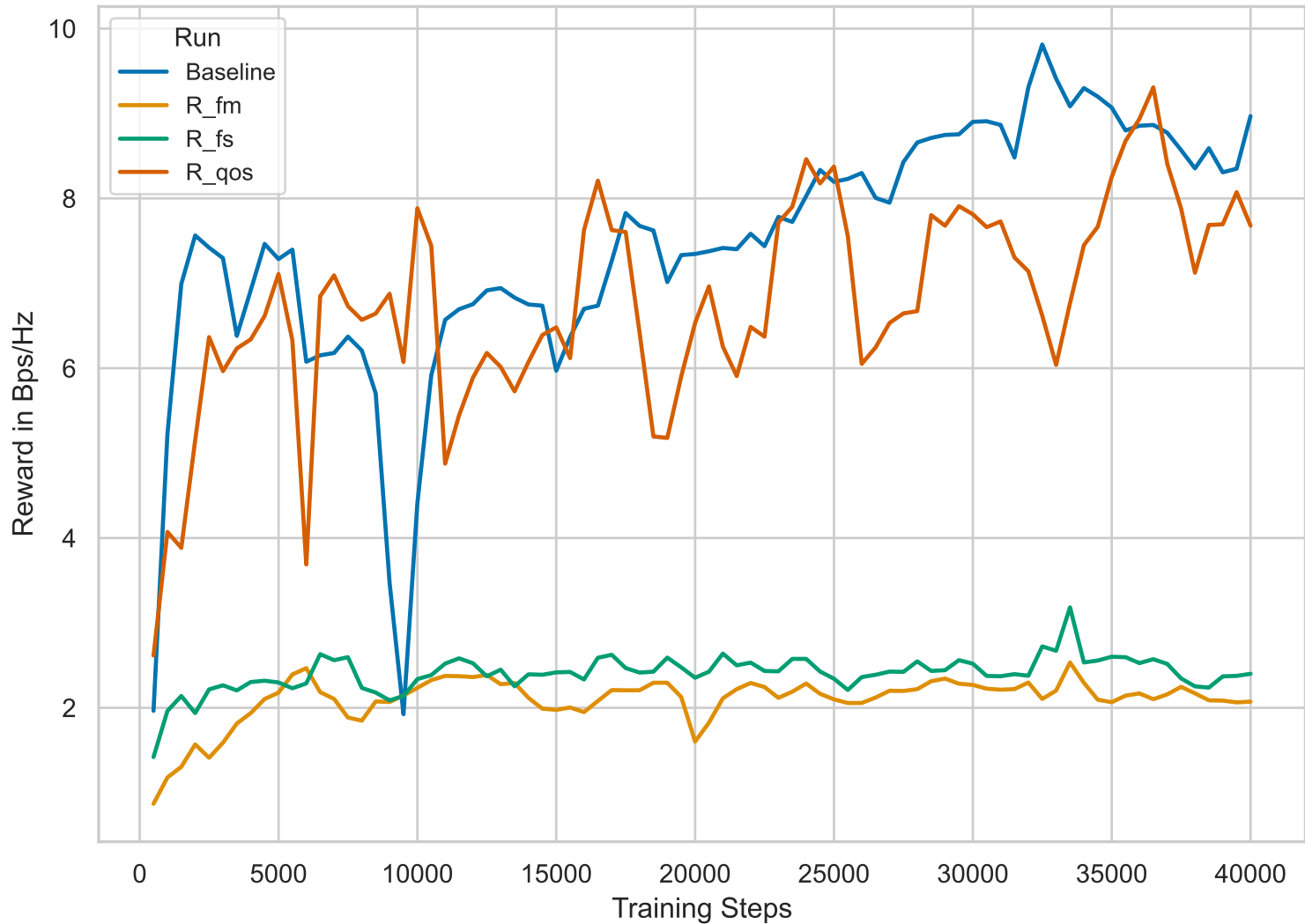
Baseline Reward Over Time (Local Average) Bps/Hz
