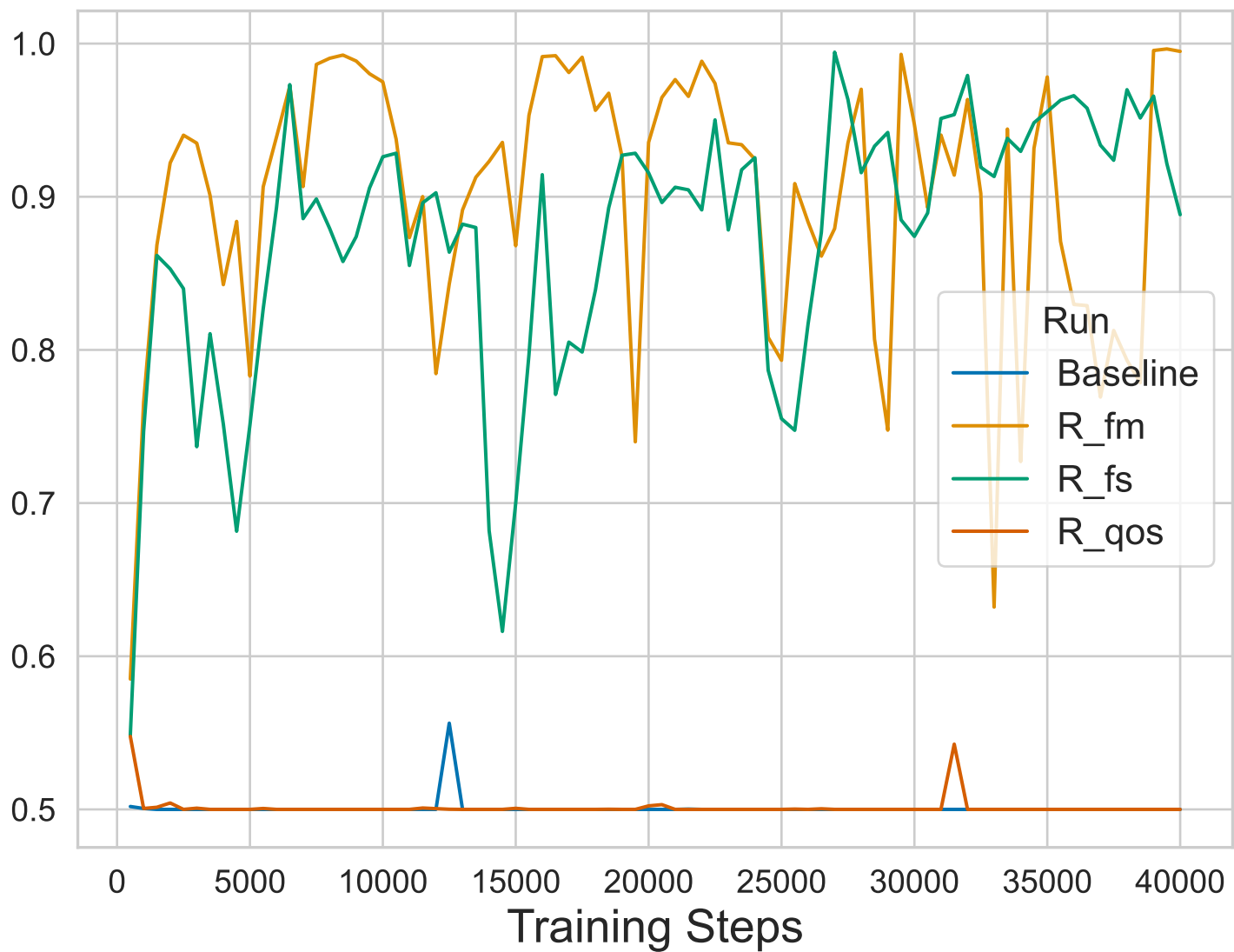
Jain Fairness Index
