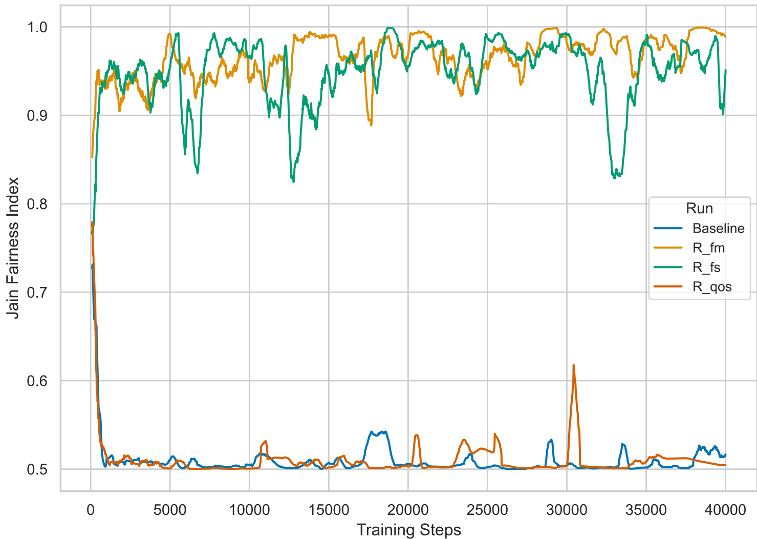
User Instant JFI Over Time
