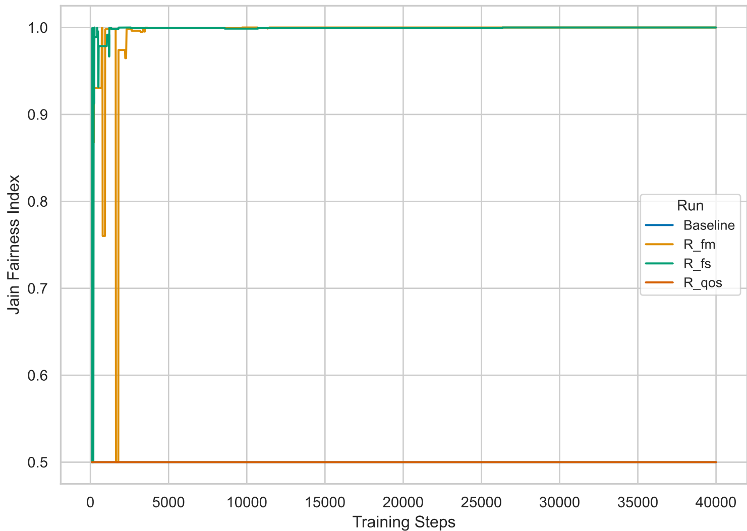
JFI for the best reward obtained
