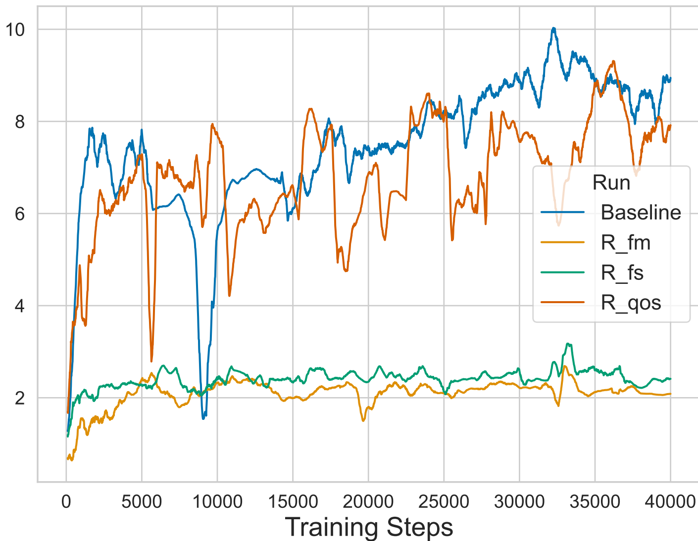
Eavesdropper Reward in Bps/Hz
