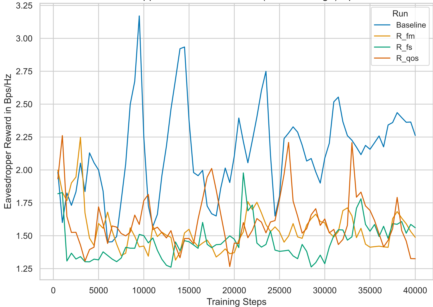
Eavesdropper Reward Over Time (Local Average) Bps/Hz
