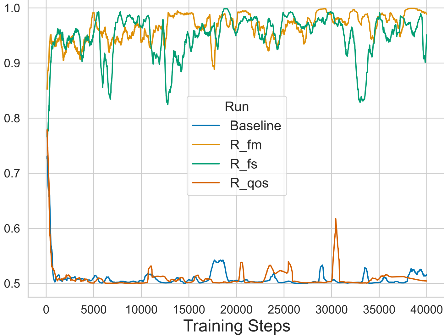
Jain Fairness Index
