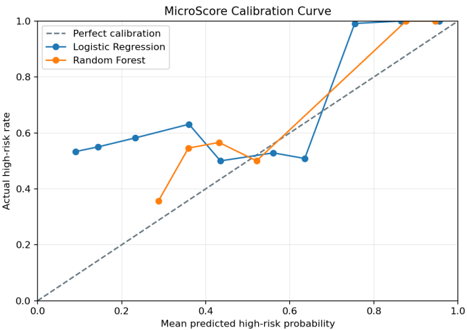
Figure 2. Calibration of held-out synthetic probabilities.
