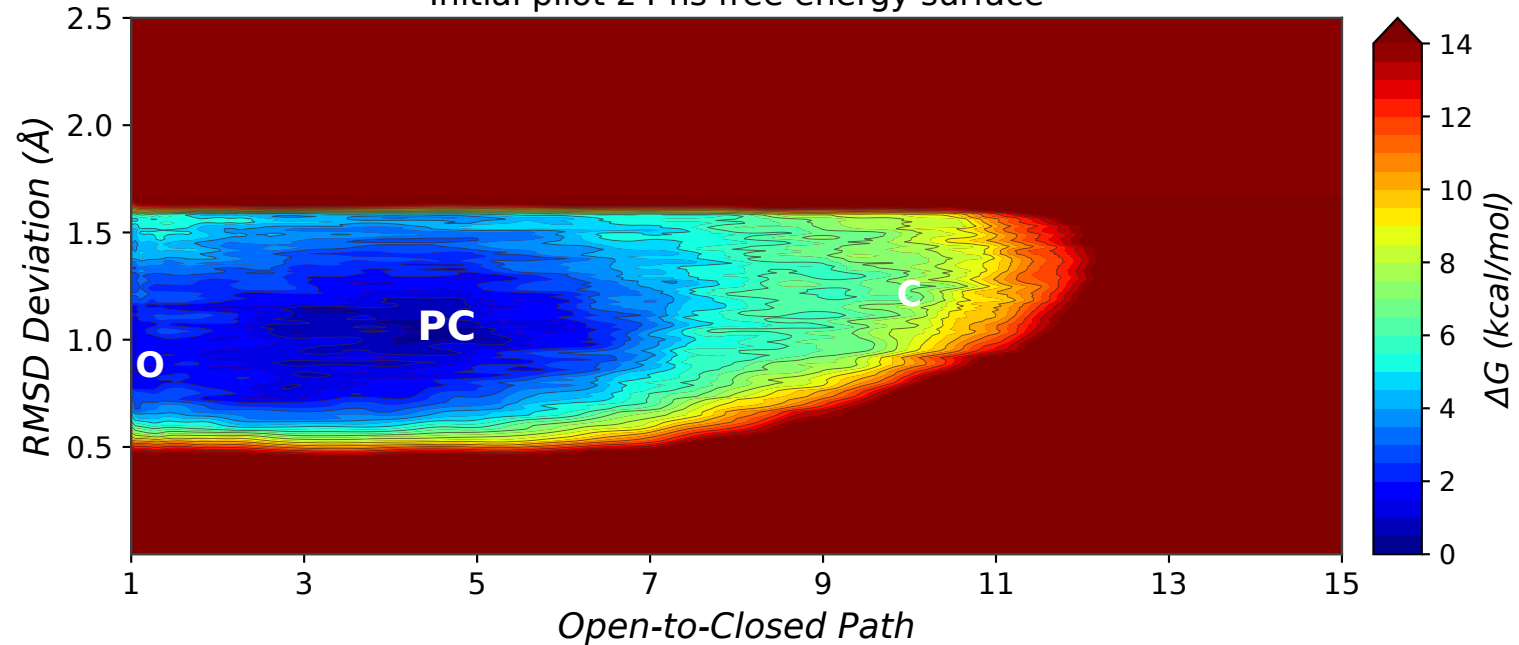
Initial pilot 24 ns free energy surface
