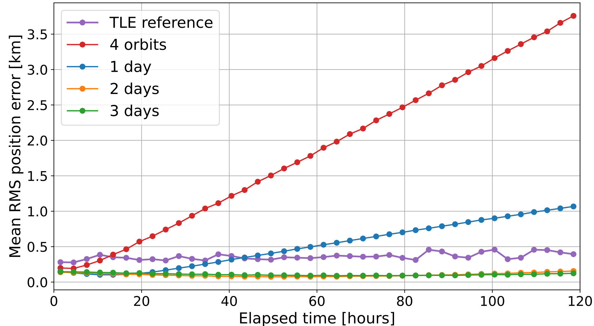
Mean RMS Position Error over all satellites
