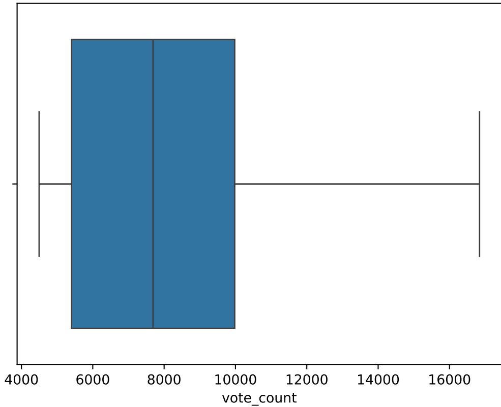
Boxplot vote_count (Excel)
