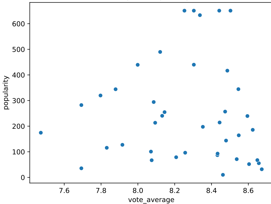
Vote Average vs Popularity (Excel)
