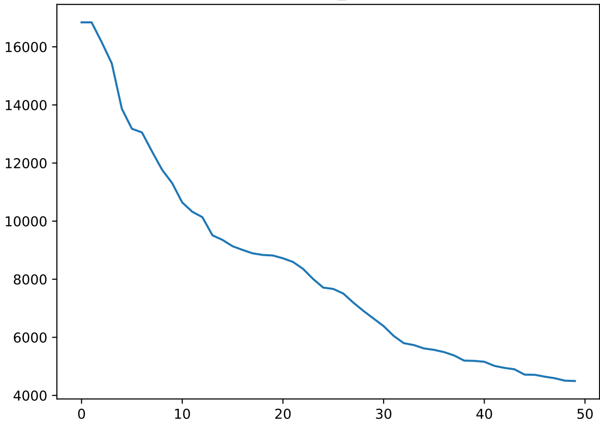
Time series vote_count (Excel)
