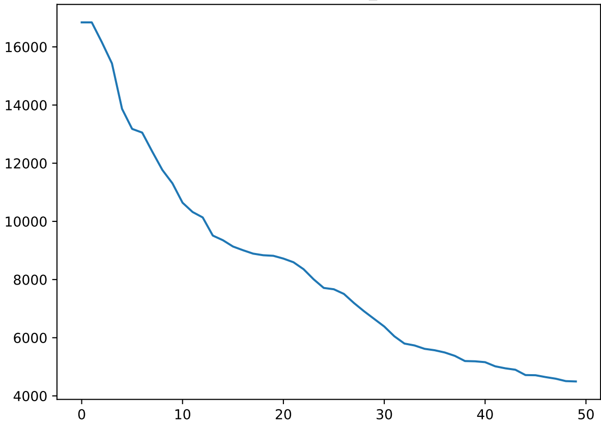
Time series vote_count
