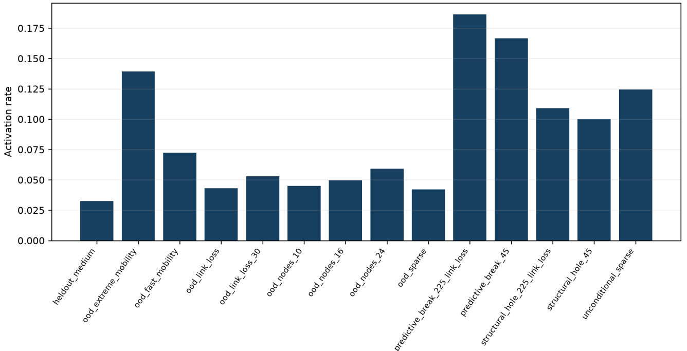
FIGURE 10. Switch activation by scenario. A switched action and the need to compute the predictive branch are different events: DiSwitch computes both branches, while Early Exit attempts to skip a branch before the switch can be fully evaluated.
