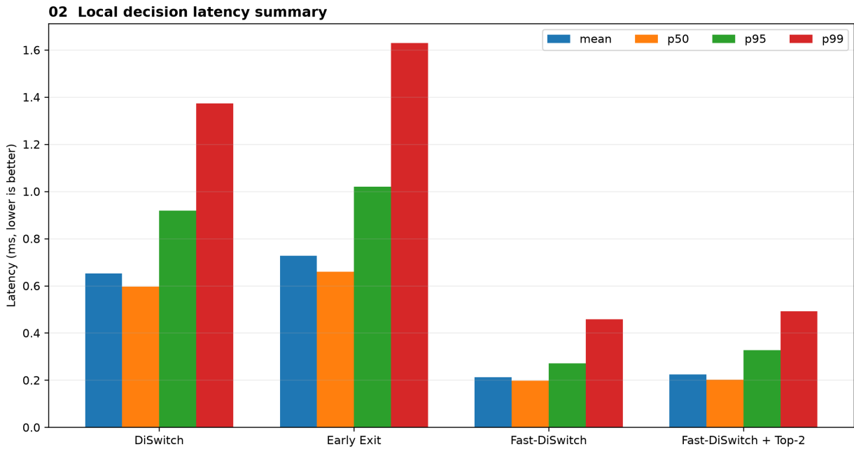
FIGURE 2. Mean, median, p95, and p99 latency summaries for DiSwitch and candidate variants. Fast-DiSwitch variants are approximate policies and require a separate reliability judgment.
