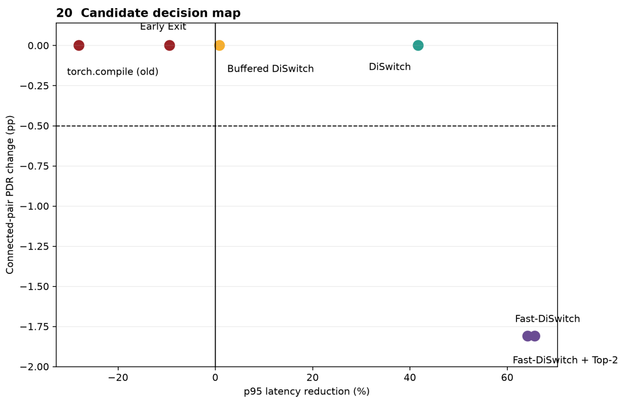
FIGURE 20. Candidate decision matrix. DiSwitch improves the duplicated legacy execution without an outcome change; buffering is too small; Early Exit is slower; Fast-DiSwitch violates the quality gate.
