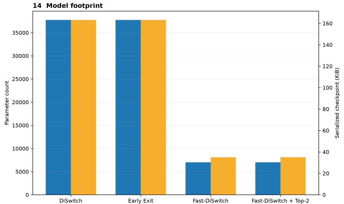
FIGURE 14. Parameter and serialized-size comparison. Early Exit shares the DiSwitch weights; Fast-DiSwitch contains 7,011 parameters and is a separately distilled approximate model.
