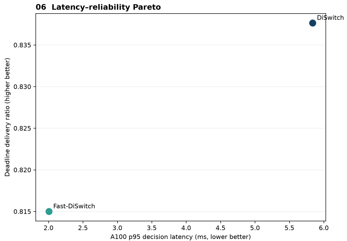
FIGURE 6. Deadline-delivery ratio versus A100 p95 decision latency. DiSwitch occupies the reliability-oriented point; Fast-DiSwitch occupies a lower-latency but lower-reliability point.
