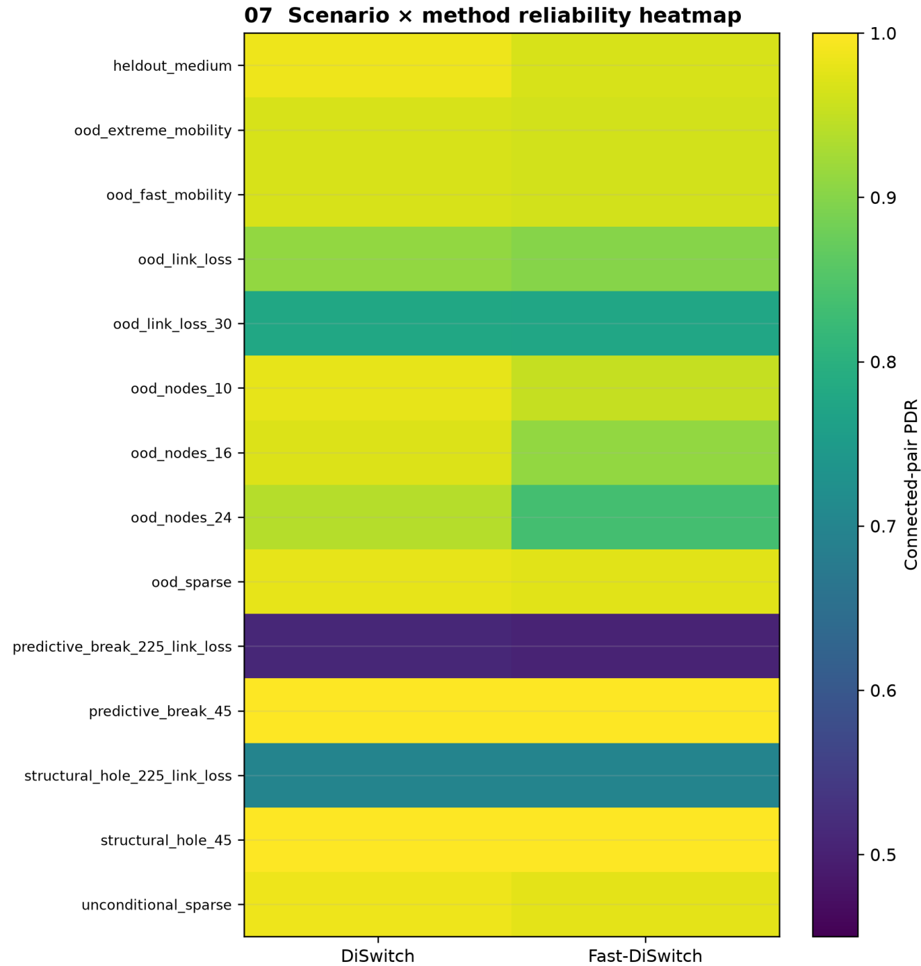
FIGURE 7. Scenario-level reliability heatmap. It reveals that Fast-DiSwitch degradation is concentrated in specific OOD node-density and predictive-break conditions rather than uniform across the benchmark.
