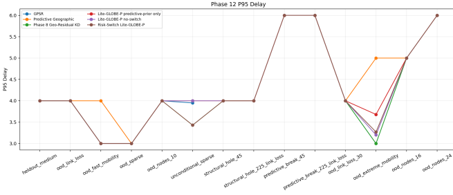
Fig. 3. Phase 12 95th-percentile packet delivery delay comparison.
