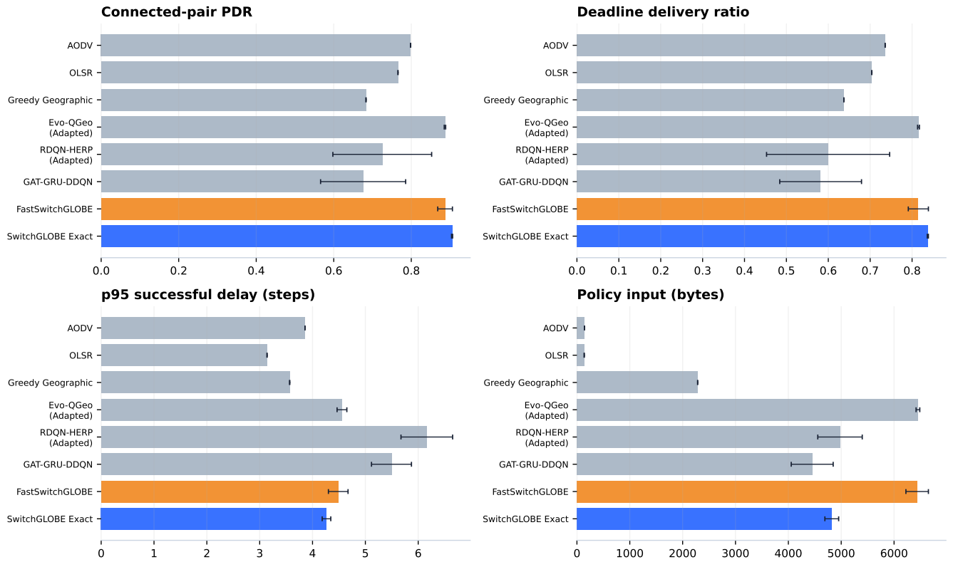
FIGURE 5. Common-simulator comparison. Error bars are five-seed 95% t intervals over scenario-macro summaries. Small input size for AODV/OLSR is not wireless routing overhead.
