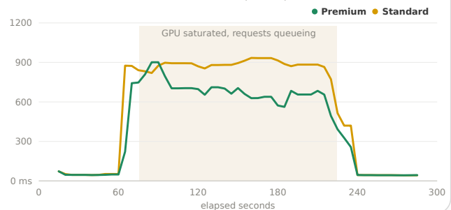
Rolling p95 TTFT by class
