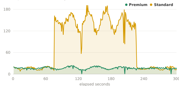
In-flight requests by class
