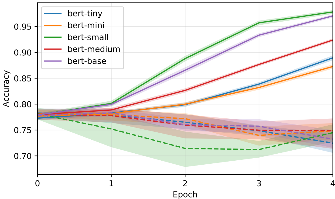
iSarcasm Dataset
