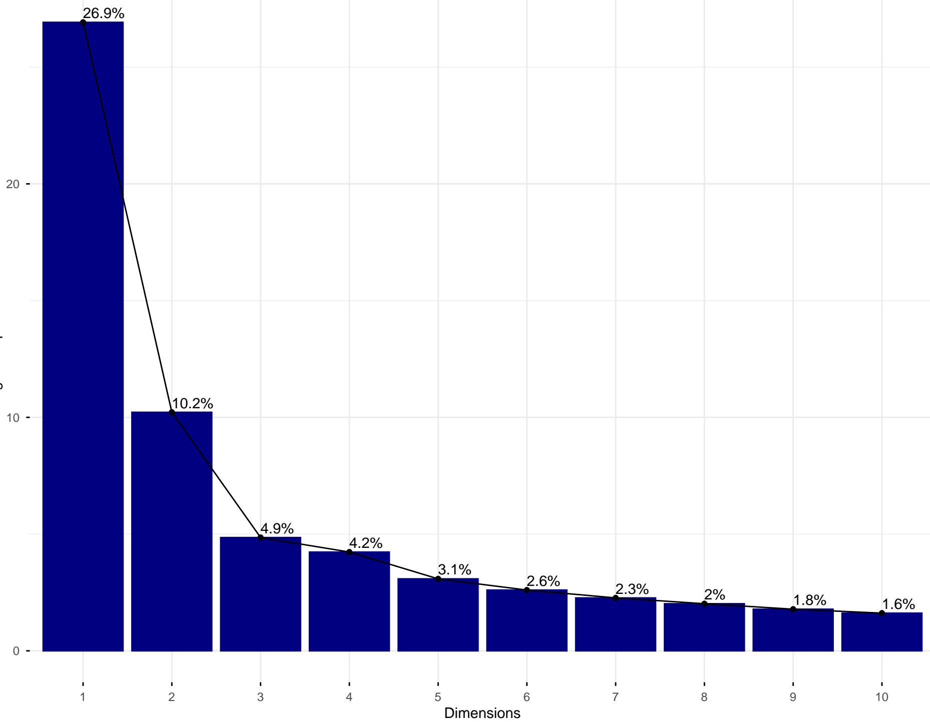
Scree plot
