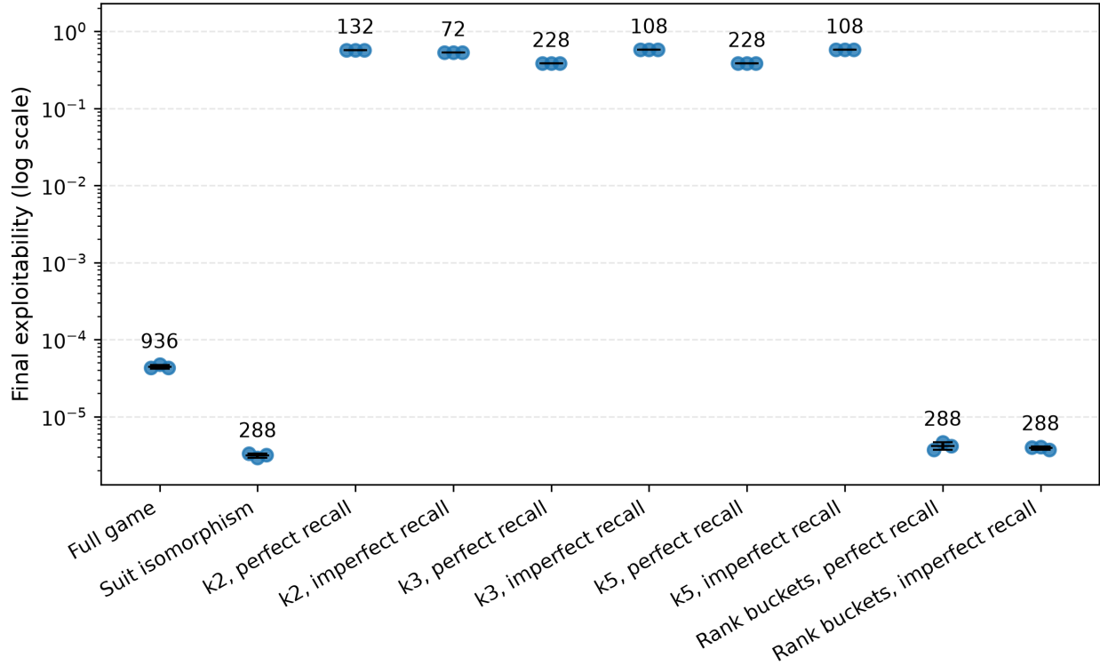
Figure 1: Fixed-limit Leduc: final exploitability after 180 s of CFR+ for each abstraction configuration (three runs, log scale); the number above each group is its information-set count.
