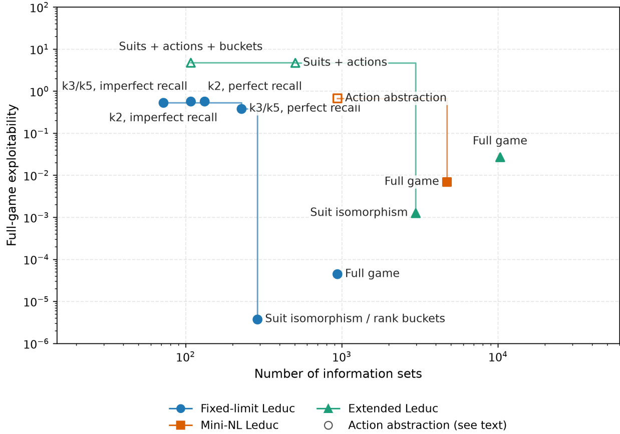
Figure 4: Pareto frontier: information-set count against full-game exploitability after 180 s of CFR+ for each abstraction configuration (mean of three runs). Lines join each game’s non-dominated points; hollow markers are action-abstraction configurations, whose values reflect the current deployment rule.
