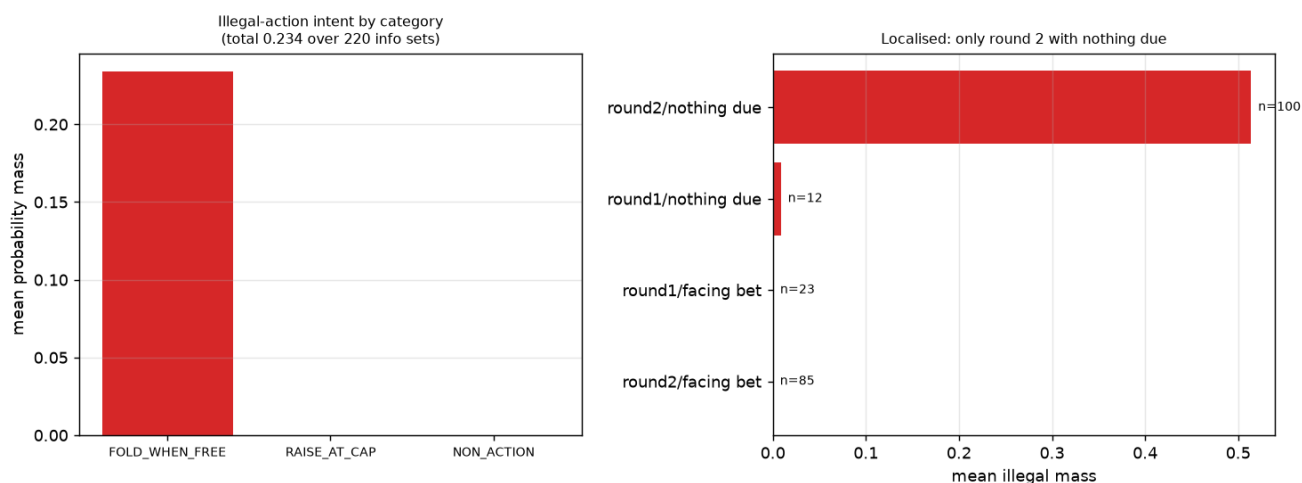
Фигура 6: Illegal-action intent by category and by situation on Ледюк Холдем.
