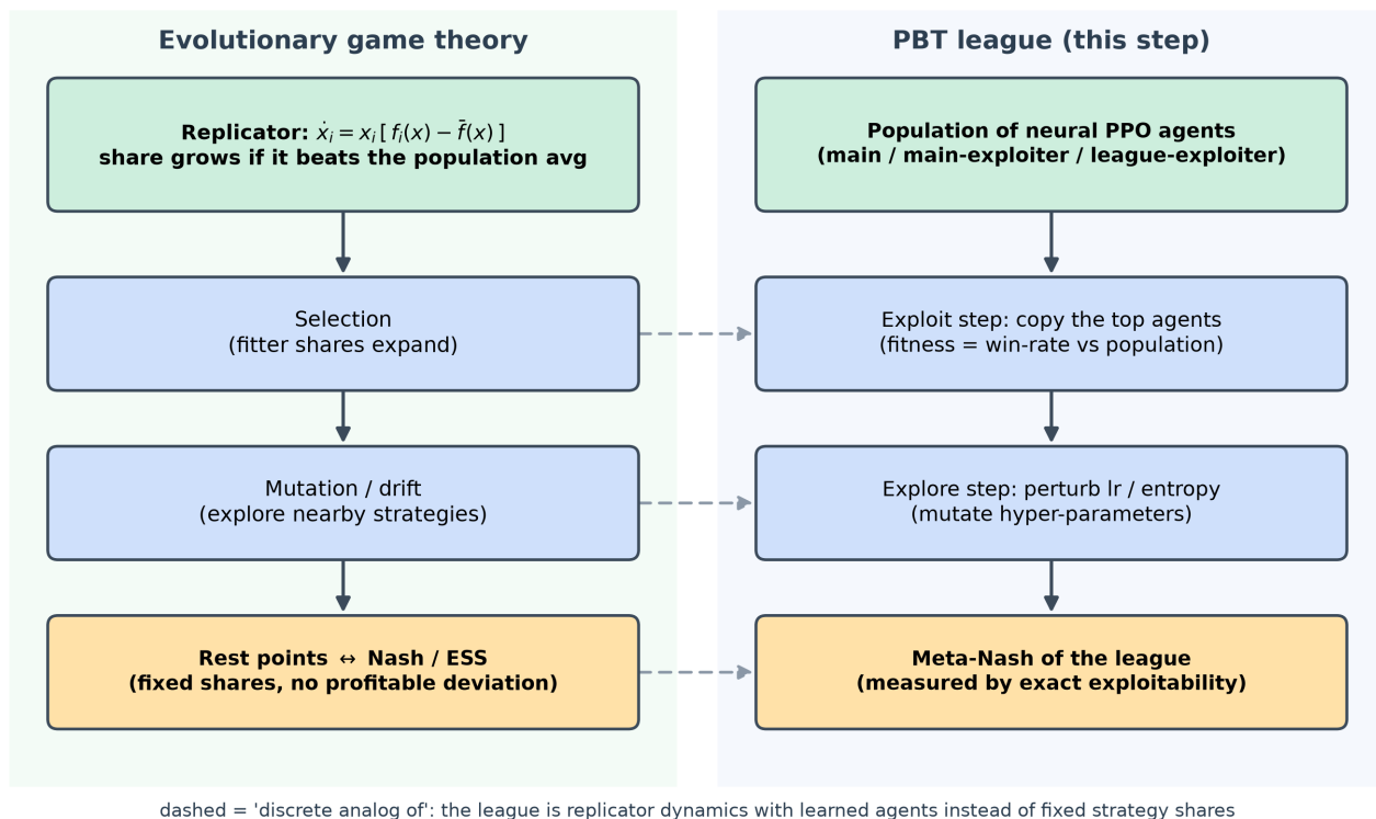
Фигура 1: Evolutionary game theory as the continuous idealization of a PBT league: replicator selection ↔ copying the fitter agents, mutation/drift ↔ perturbing learning rate and entropy, and replicator rest points ↔ the meta-Nash / ESS the league is trying to reach. The league is replicator dynamics with learned agents instead of fixed strategy shares.
