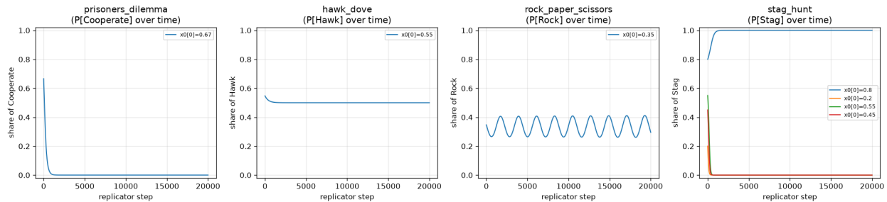
Фигура 1: Replicator phase portraits on the four matrix games: Prisoner's Dilemma collapses to all-Defect, Hawk-Dove converges to the interior 0.5 ESS, Rock-Paper-Scissors orbits the centre without converging, and Stag Hunt splits into two basins (all-Stag or all-Hare) depending on the start. The non-converging RPS orbit is the visceral case for the diversity machinery in Part II.
