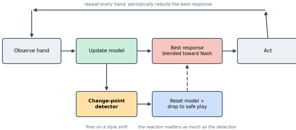
Figure 7: The adaptive exploitation loop: observe, update the model, best-response (blended toward Nash for safety), and act; a change-point detector can reset the model when the opponent’s style shifts.
