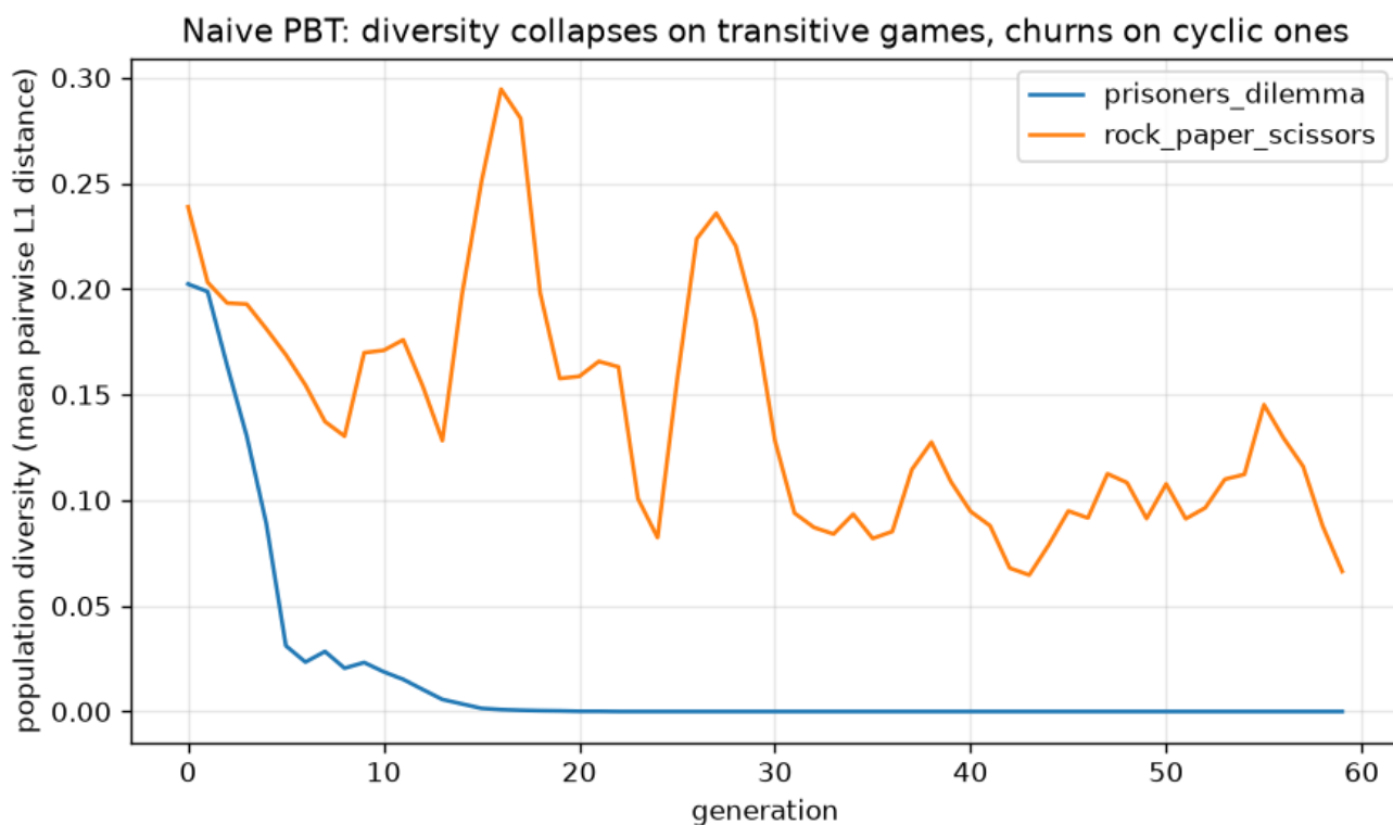
Фигура 7: Mini-PBT diversity: on the transitive Prisoner’s Dilemma the population collapses to a single strategy (diversity → 0), while on cyclic Rock-Paper-Scissors it churns indefinitely (0.07-0.29) as it chases the wheel of counters. Game structure, not population size, decides whether diversity survives.
