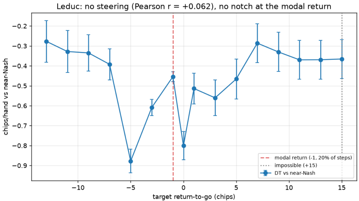
Фигура 7: DT performance against the conditioned target return on Leduc, with standard errors. There is no collapse at the modal return and no monotone trend.
