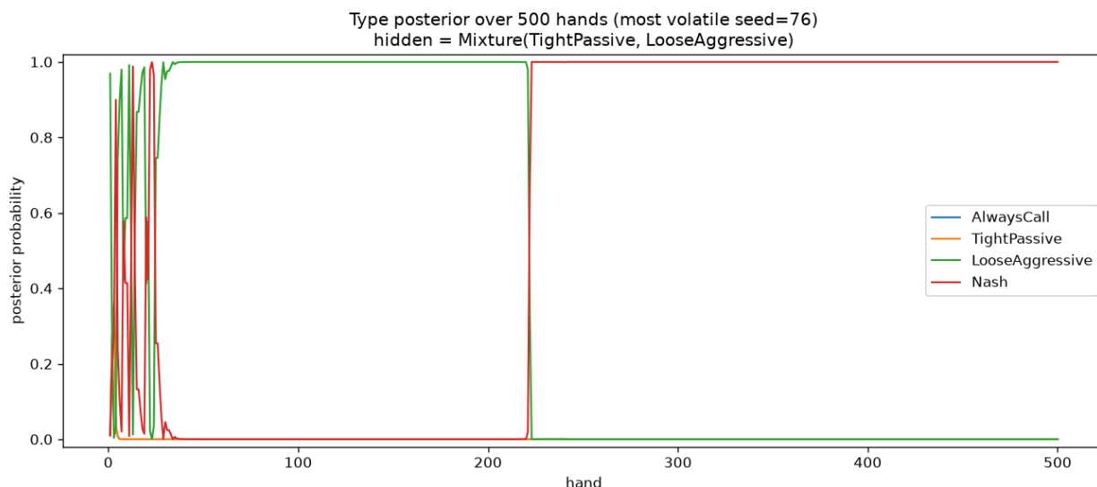
Фигура 21: Hidden = Mixture, 500 hands (most volatile seed): a wrong type can dominate for 200 hands before Nash overtakes; once locked, Nash never falls.
