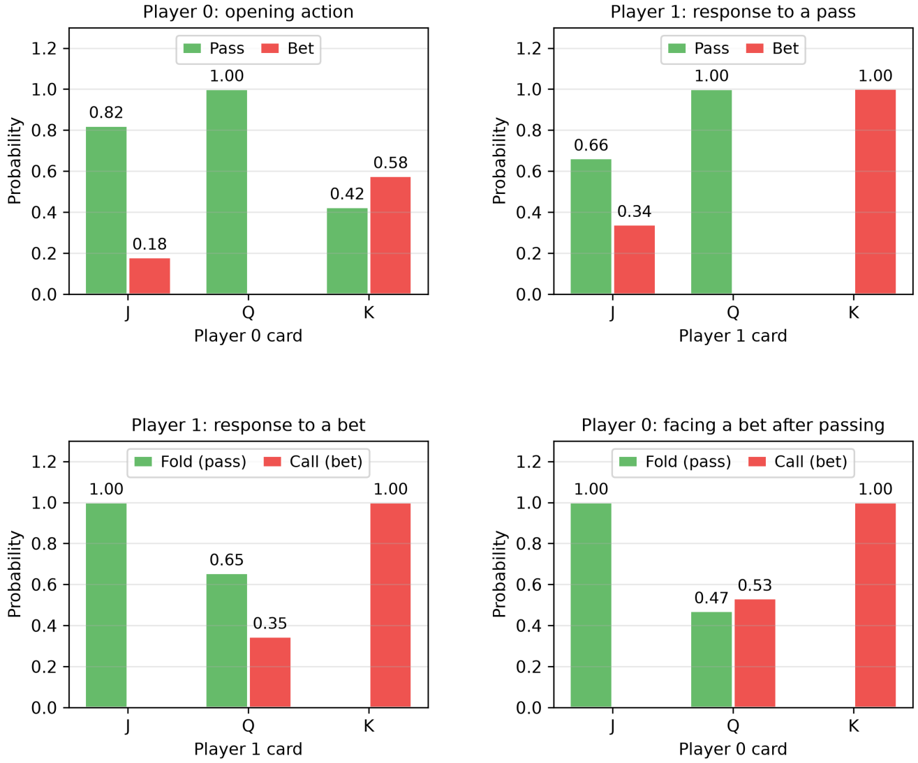
Figure 3: The average strategy CFR finds for Kuhn poker after 100,000 iterations: action probabilities at each information set. The Jack's bluffing and the Queen's calling frequencies are close to the Nash equilibrium family ( \alpha \approx 0.18 ).
