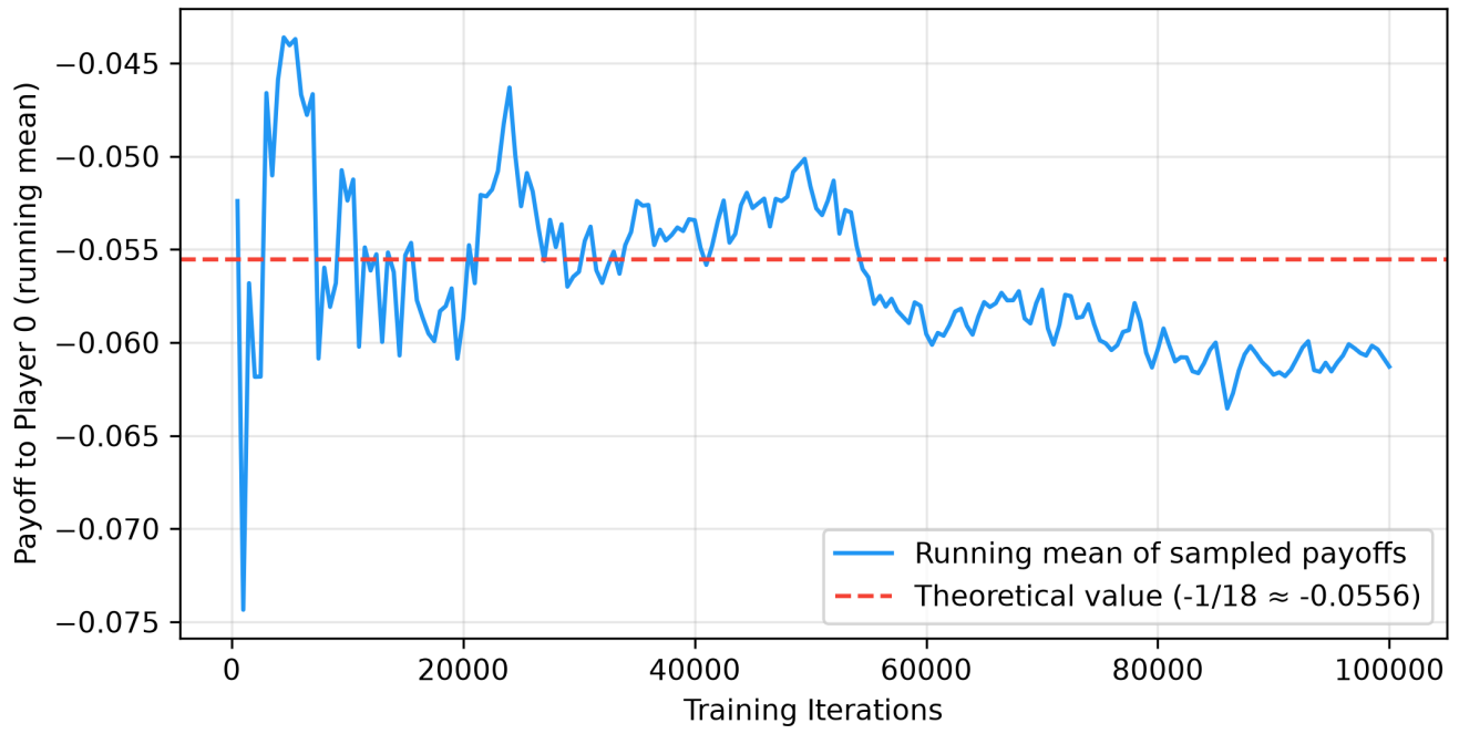
Figure 1: The running mean of Player 0's payoff over the sampled deals, averaged from the start of training, fluctuates around the theoretical value -1/18 within sampling noise. The exact value of the average strategy after 100,000 iterations is -0.0555 .
