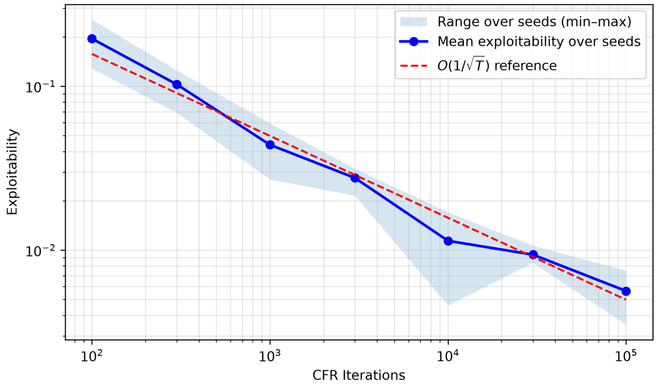
Figure 2: Exploitability of the average strategy against the number of iterations, log-log scale, mean over five seeds; the shaded band is their range. The measured points roughly follow the O(1/\sqrt{T}) reference slope (dashed line), consistent with the theoretical bound.
