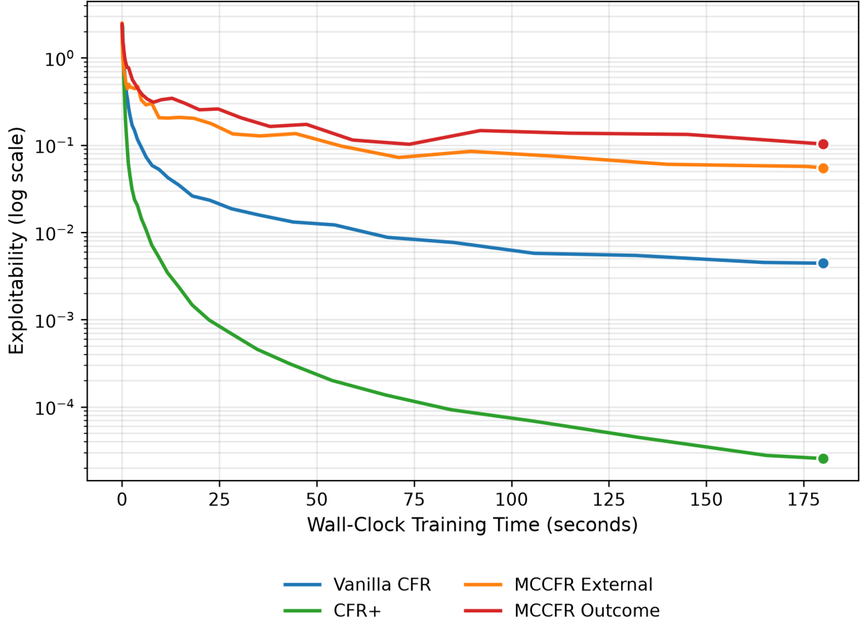
Figure 6: Exploitability vs Wall-Clock Time (log-y)
