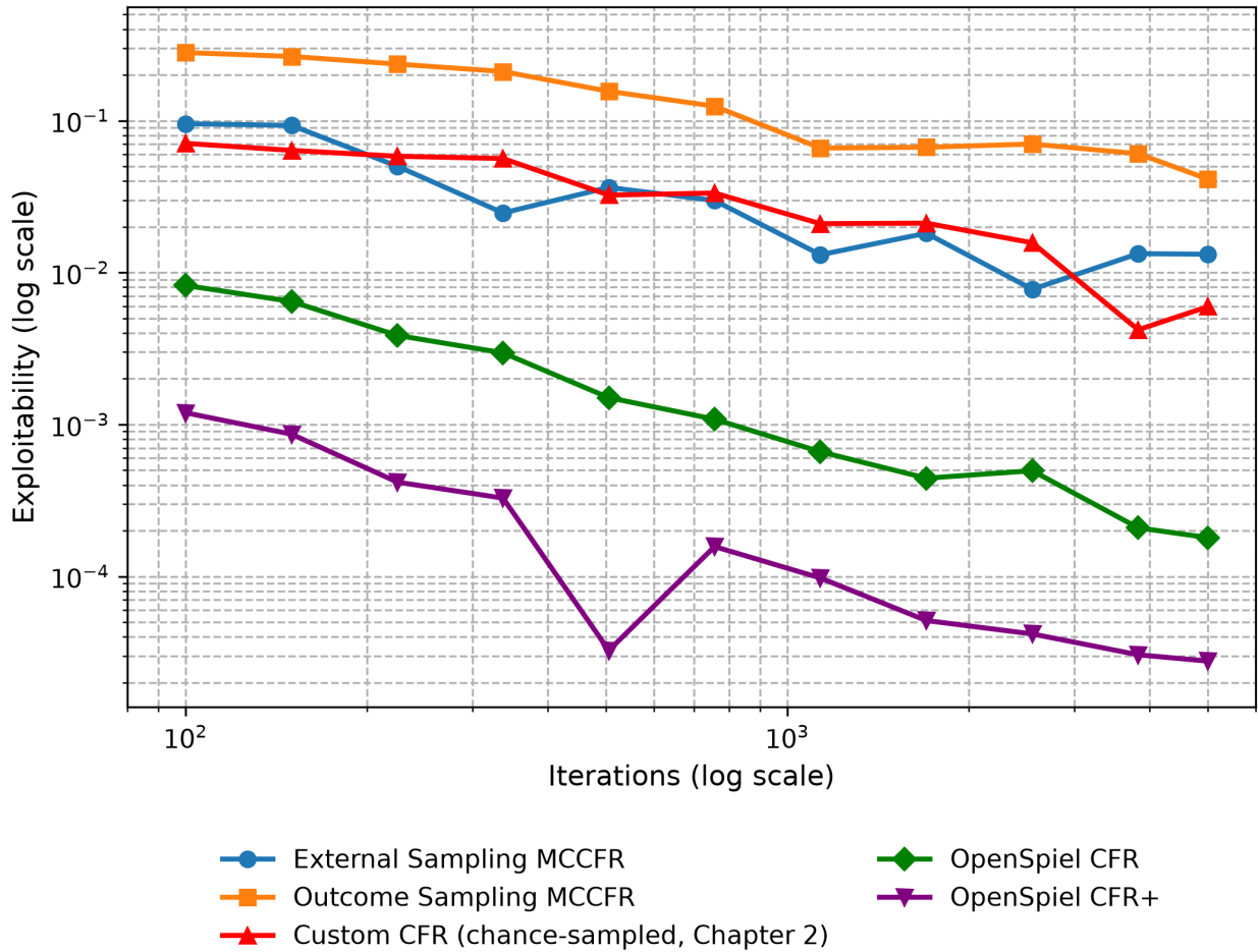
Figure 1: Kuhn — Exploitability vs Iterations
