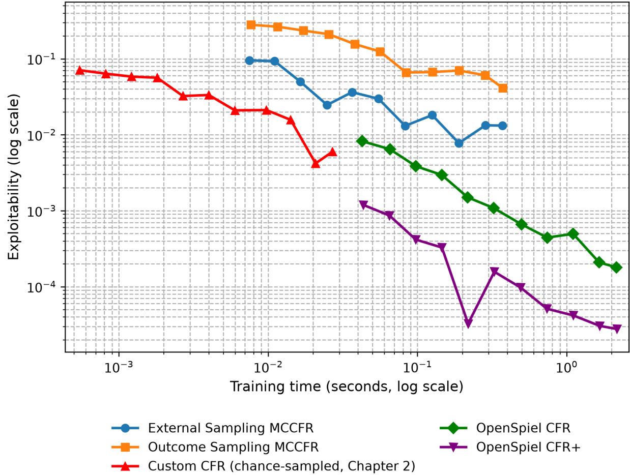
Figure 2: Kuhn — Exploitability vs Training Time
