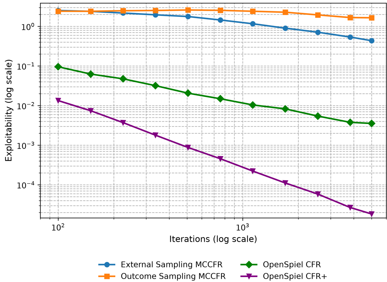
Figure 3: Leduc — Exploitability vs Iterations
