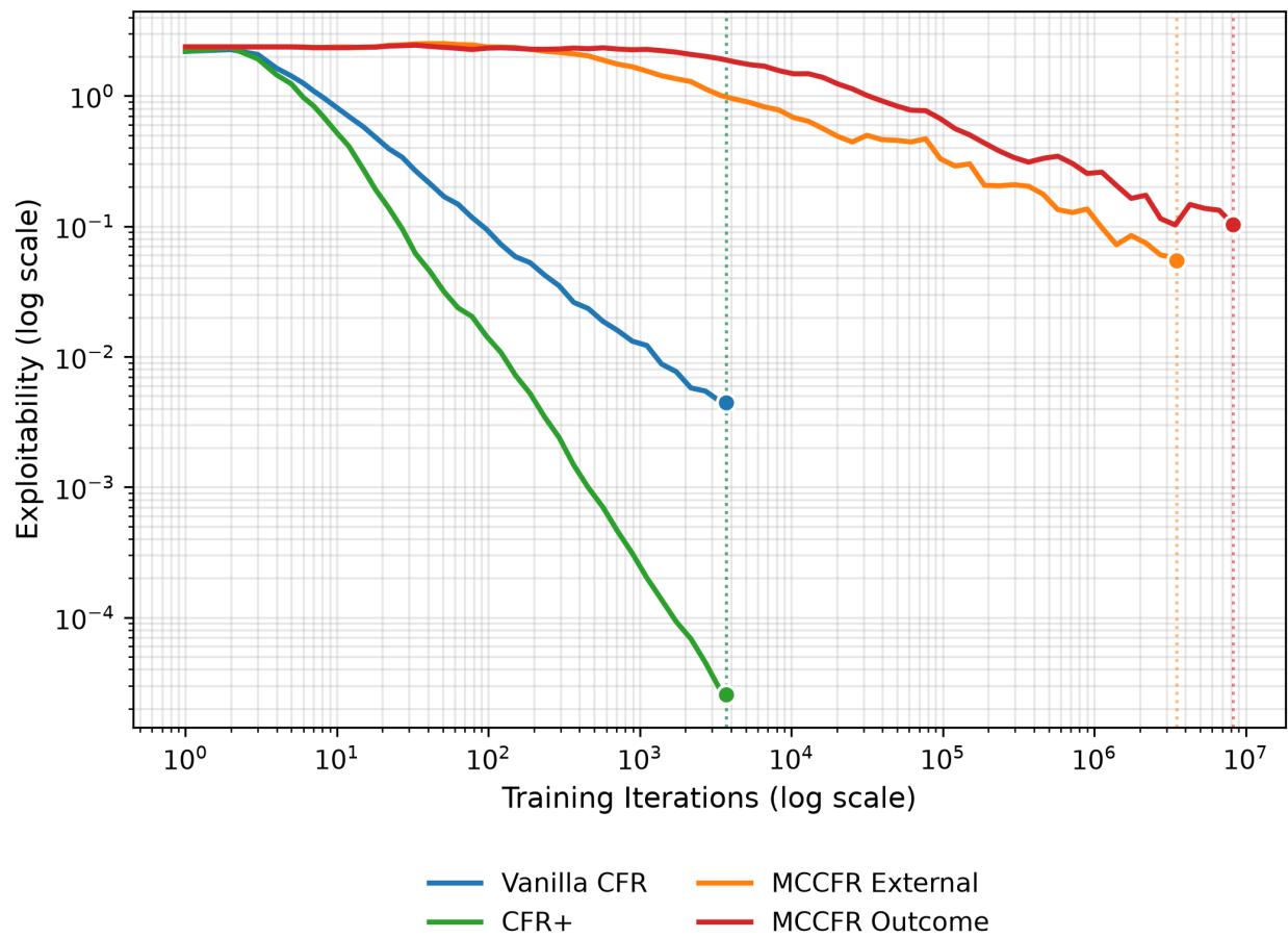
Figure 5: Exploitability vs Iterations (log-log)
