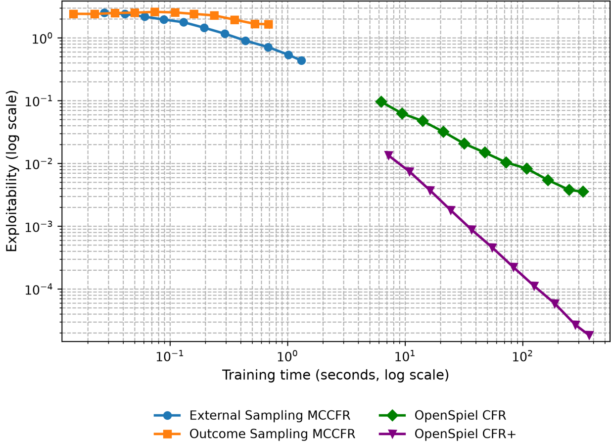
Figure 4: Leduc — Exploitability vs Training Time
